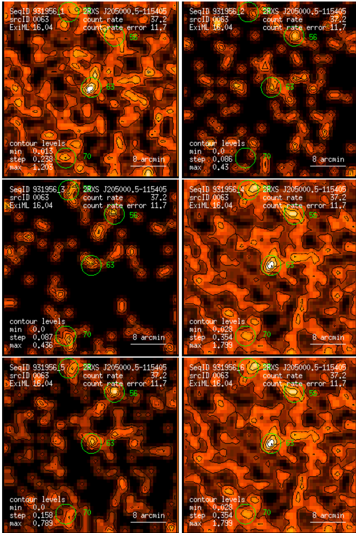
Figure 63: RASS 931956: detection 0063: band rate images, Gaussian filter: (1) PSPC channels 11 – 41, (2) 52 – 90, (3) 91 – 201, (4) 11 – 235, (5) 52 – 201, (6) 11 – 201. Broad band rates in counts/ks. Band rate contour levels in counts/ks/arcmin 2 .
