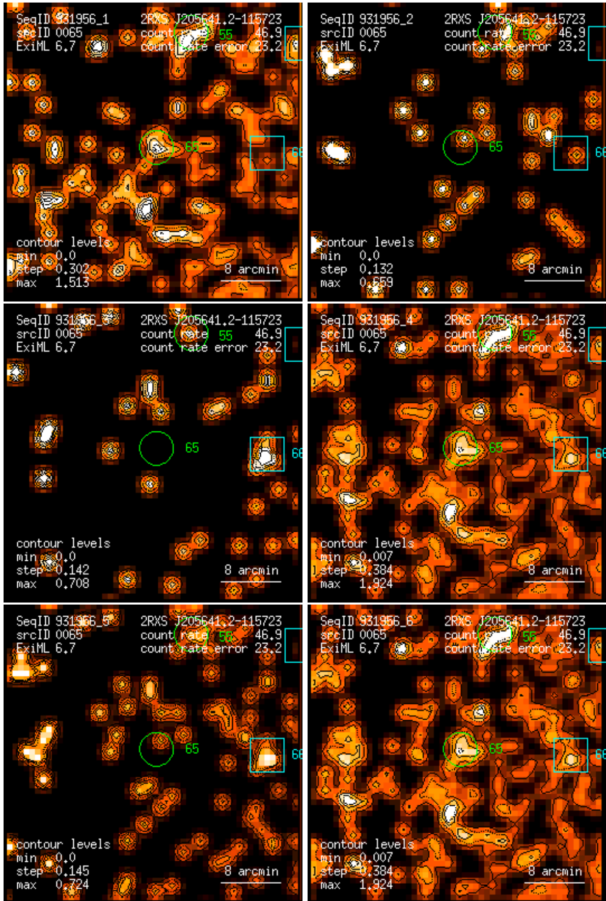
Figure 65: RASS 931956: detection 0065: band rate images, Gaussian filter: (1) PSPC channels 11 – 41, (2) 52 – 90, (3) 91 – 201, (4) 11 – 235, (5) 52 – 201, (6) 11 – 201. Broad band rates in counts/ks. Band rate contour levels in counts/ks/arcmin 2 .
