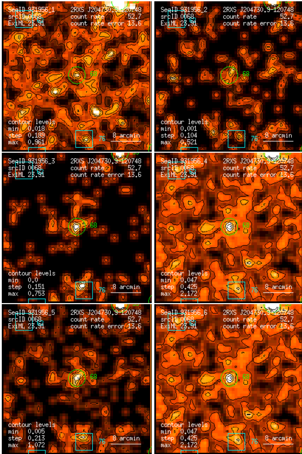
Figure 68: RASS 931956: detection 0068: band rate images, Gaussian filter: (1) PSPC channels 11 – 41, (2) 52 – 90, (3) 91 – 201, (4) 11 – 235, (5) 52 – 201, (6) 11 – 201. Broad band rates in counts/ks. Band rate contour levels in counts/ks/arcmin 2 .
