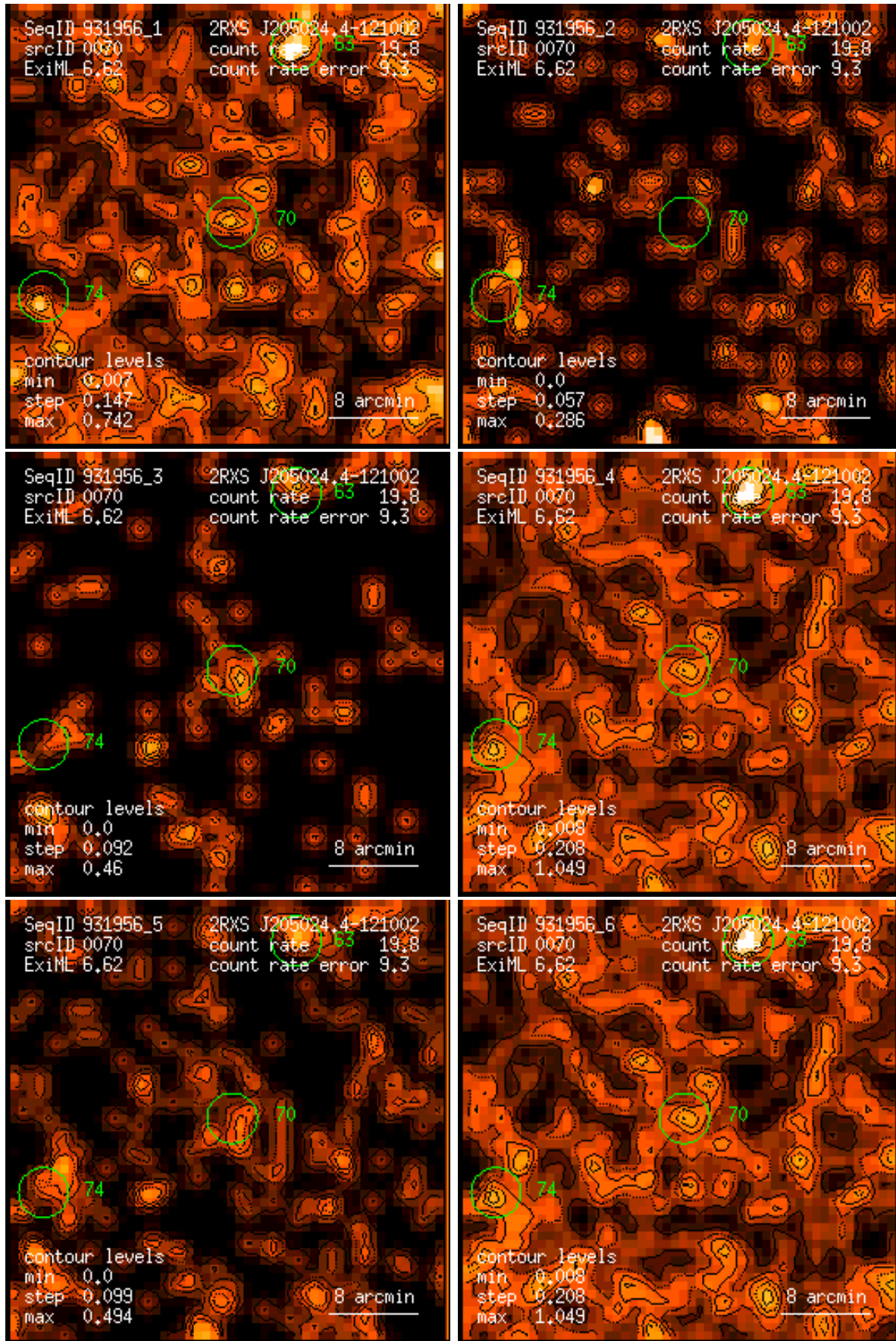
Figure 70: RASS 931956: detection 0070: band rate images, Gaussian filter: (1) PSPC channels 11 – 41, (2) 52 – 90, (3) 91 – 201, (4) 11 – 235, (5) 52 – 201, (6) 11 – 201. Broad band rates in counts/ks. Band rate contour levels in counts/ks/arcmin 2 .
