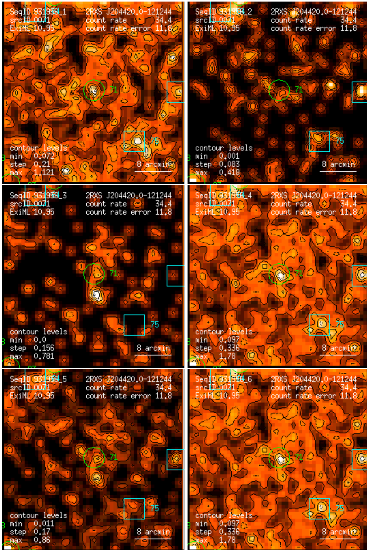
Figure 71: RASS 931956: detection 0071: band rate images, Gaussian filter: (1) PSPC channels 11 – 41, (2) 52 – 90, (3) 91 – 201, (4) 11 – 235, (5) 52 – 201, (6) 11 – 201. Broad band rates in counts/ks. Band rate contour levels in counts/ks/arcmin 2 .
