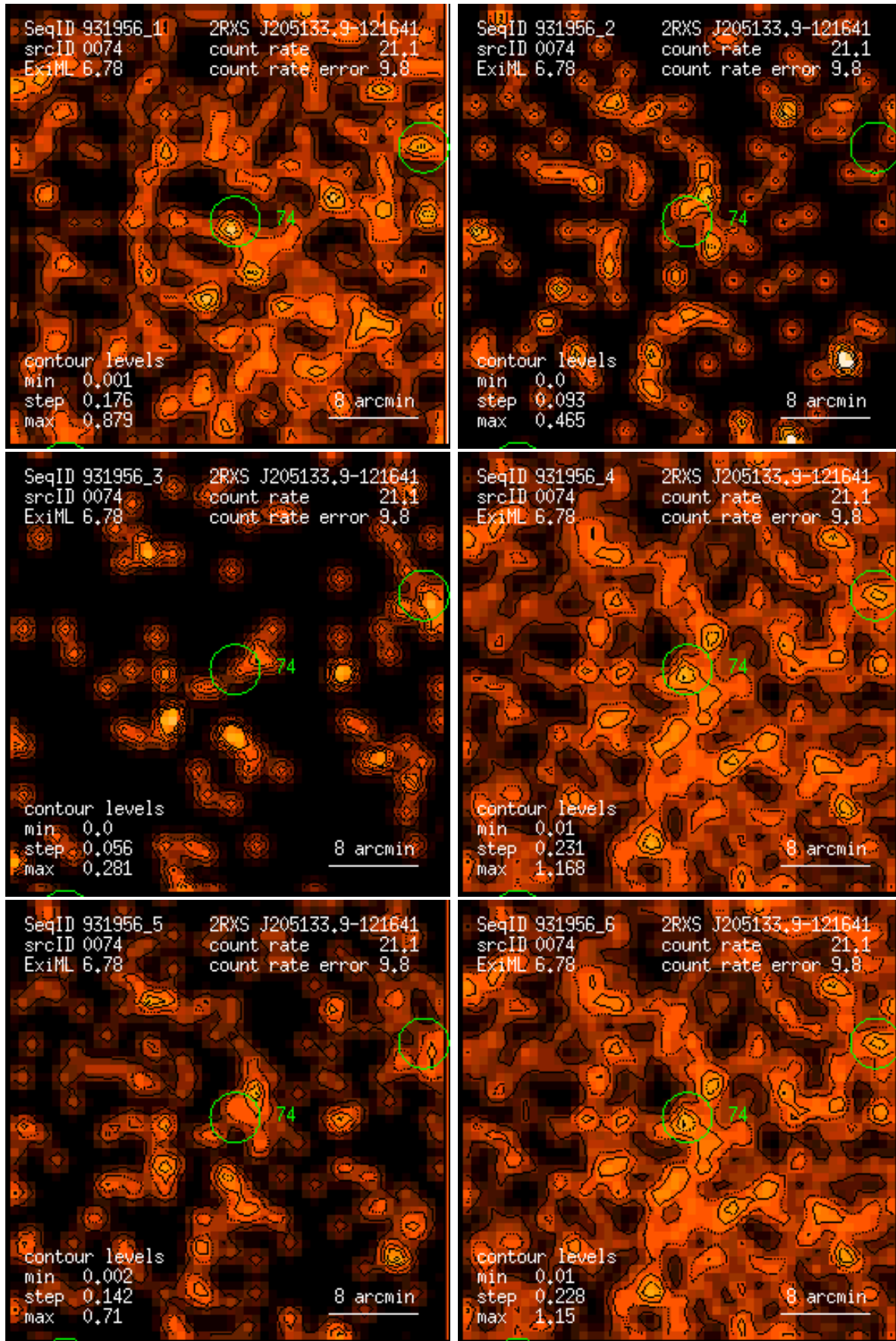
Figure 74: RASS 931956: detection 0074: band rate images, Gaussian filter: (1) PSPC channels 11 – 41, (2) 52 – 90, (3) 91 – 201, (4) 11 – 235, (5) 52 – 201, (6) 11 – 201. Broad band rates in counts/ks. Band rate contour levels in counts/ks/arcmin 2 .
