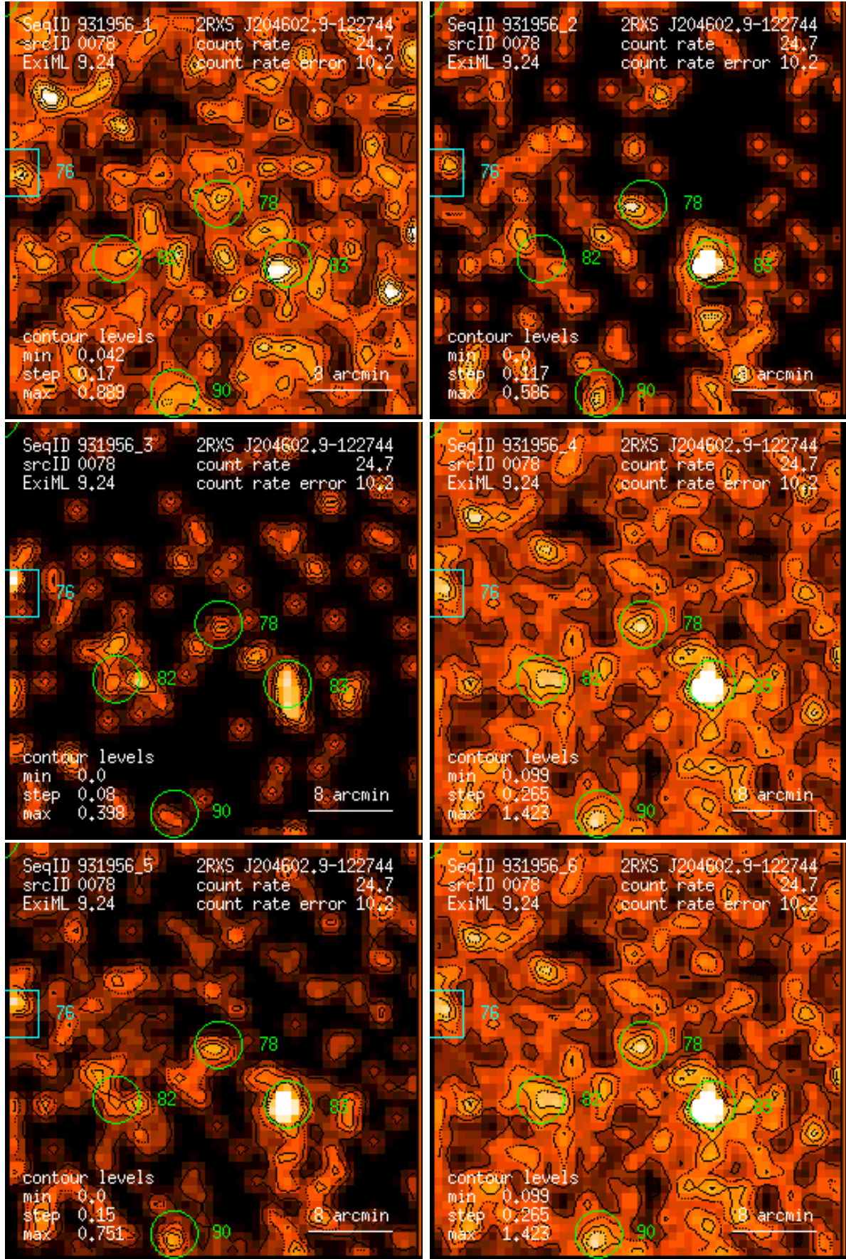
Figure 78: RASS 931956: detection 0078: band rate images, Gaussian filter: (1) PSPC channels 11 – 41, (2) 52 – 90, (3) 91 – 201, (4) 11 – 235, (5) 52 – 201, (6) 11 – 201. Broad band rates in counts/ks. Band rate contour levels in counts/ks/arcmin 2 .
