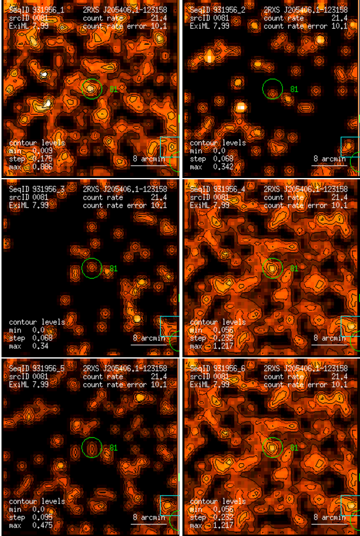
Figure 81: RASS 931956: detection 0081: band rate images, Gaussian filter: (1) PSPC channels 11 – 41, (2) 52 – 90, (3) 91 – 201, (4) 11 – 235, (5) 52 – 201, (6) 11 – 201. Broad band rates in counts/ks. Band rate contour levels in counts/ks/arcmin 2 .
