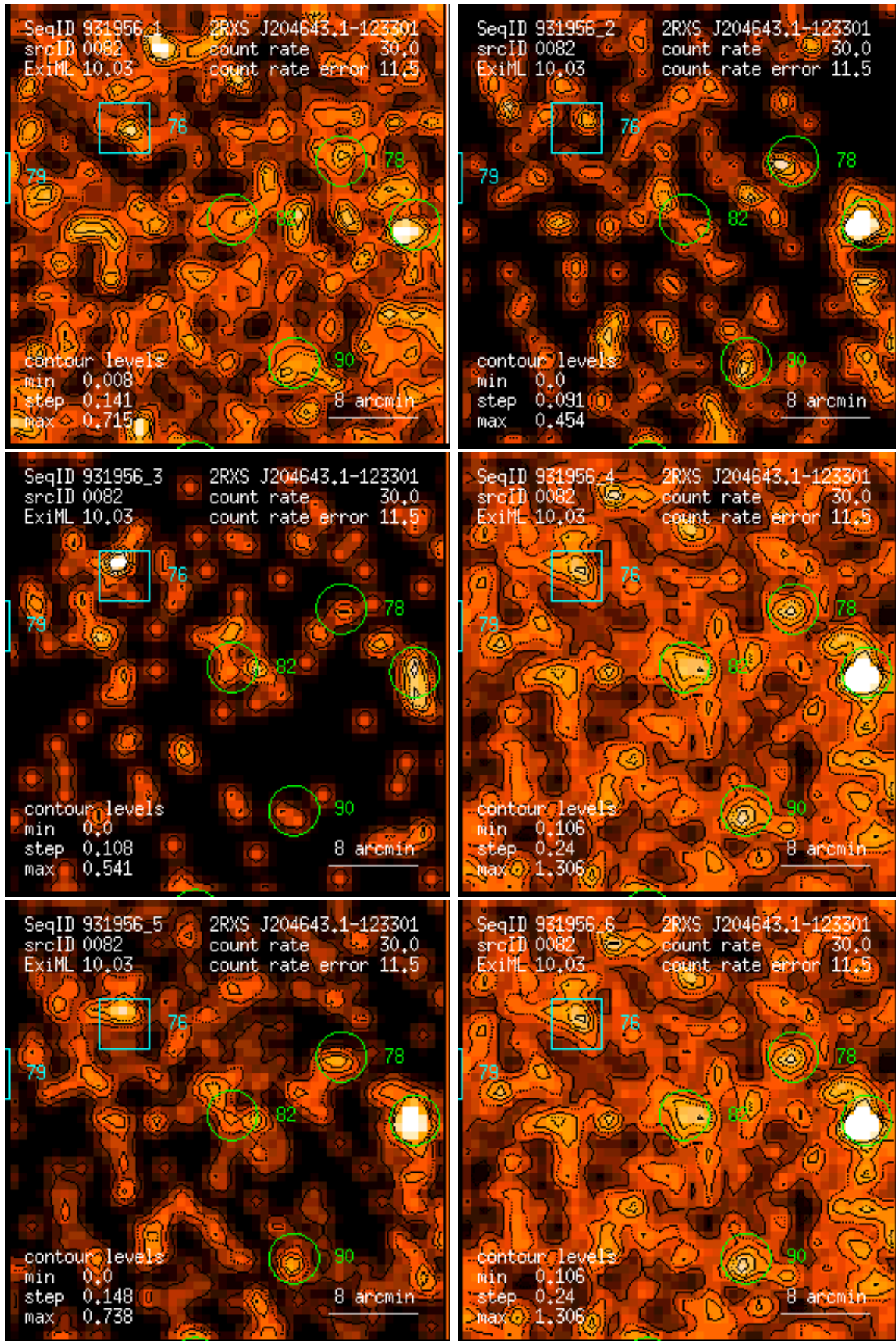
Figure 82: RASS 931956: detection 0082: band rate images, Gaussian filter: (1) PSPC channels 11 – 41, (2) 52 – 90, (3) 91 – 201, (4) 11 – 235, (5) 52 – 201, (6) 11 – 201. Broad band rates in counts/ks. Band rate contour levels in counts/ks/arcmin 2 .
