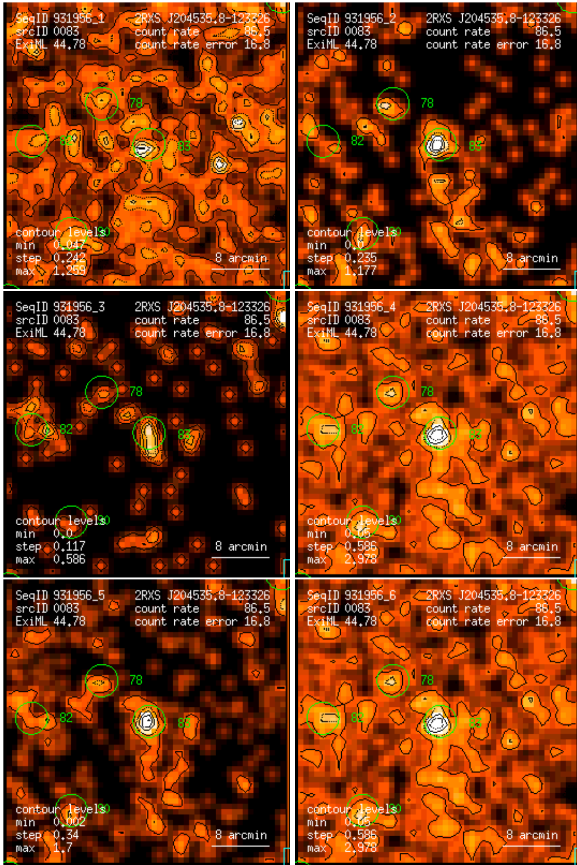
Figure 83: RASS 931956: detection 0083: band rate images, Gaussian filter: (1) PSPC channels 11 – 41, (2) 52 – 90, (3) 91 – 201, (4) 11 – 235, (5) 52 – 201, (6) 11 – 201. Broad band rates in counts/ks. Band rate contour levels in counts/ks/arcmin 2 .
