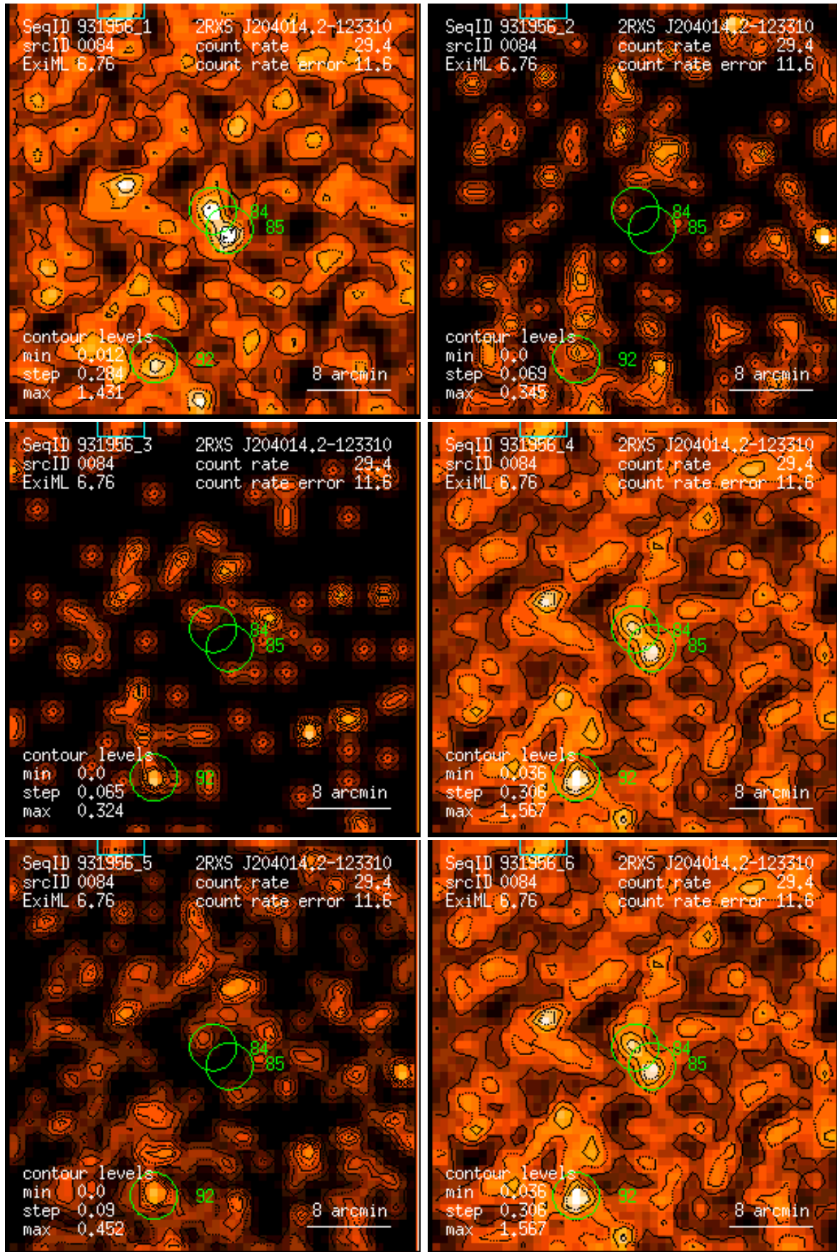
Figure 84: RASS 931956: detection 0084: band rate images, Gaussian filter: (1) PSPC channels 11 – 41, (2) 52 – 90, (3) 91 – 201, (4) 11 – 235, (5) 52 – 201, (6) 11 – 201. Broad band rates in counts/ks. Band rate contour levels in counts/ks/arcmin 2 .
