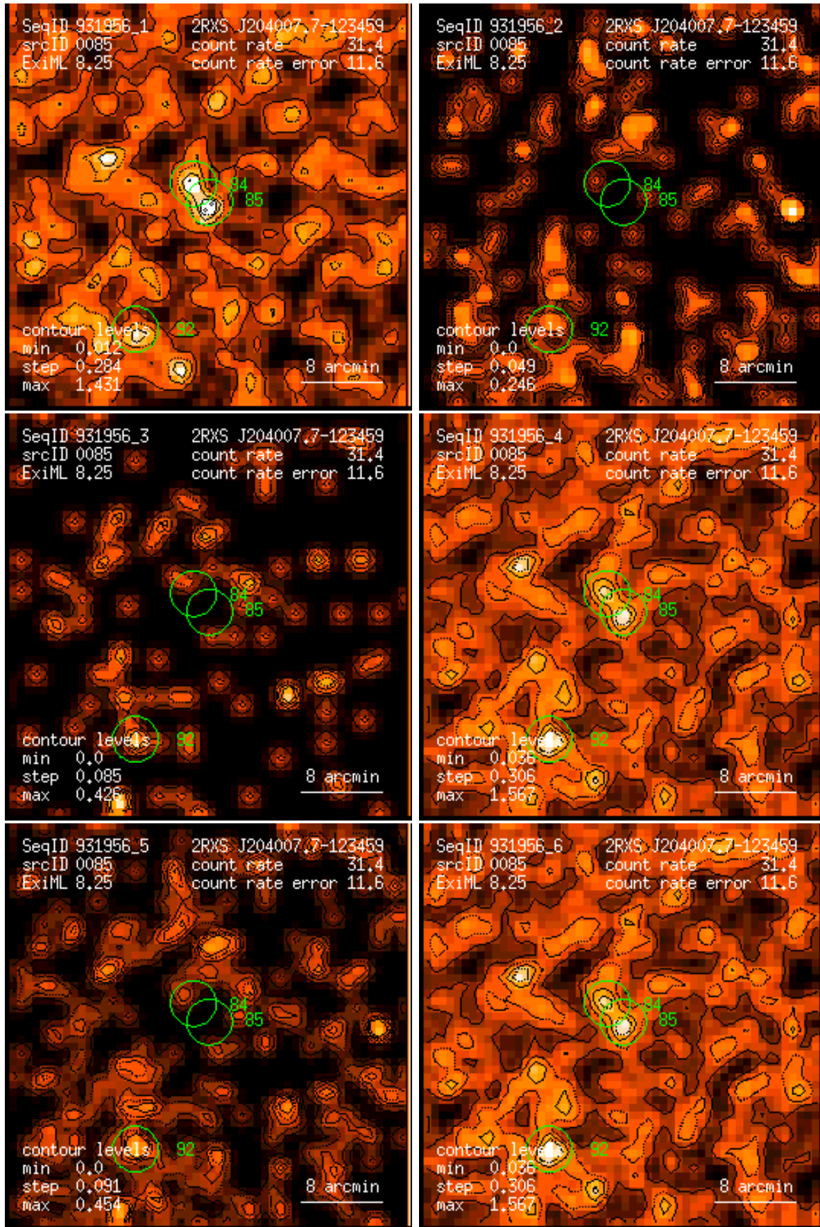
Figure 85: RASS 931956: detection 0085: band rate images, Gaussian filter: (1) PSPC channels 11 – 41, (2) 52 – 90, (3) 91 – 201, (4) 11 – 235, (5) 52 – 201, (6) 11 – 201. Broad band rates in counts/ks. Band rate contour levels in counts/ks/arcmin 2 .
