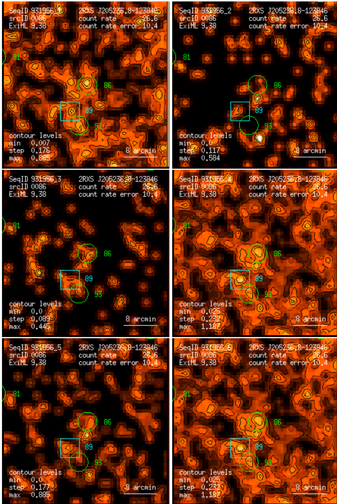
Figure 86: RASS 931956: detection 0086: band rate images, Gaussian filter: (1) PSPC channels 11 – 41, (2) 52 – 90, (3) 91 – 201, (4) 11 – 235, (5) 52 – 201, (6) 11 – 201. Broad band rates in counts/ks. Band rate contour levels in counts/ks/arcmin 2 .
