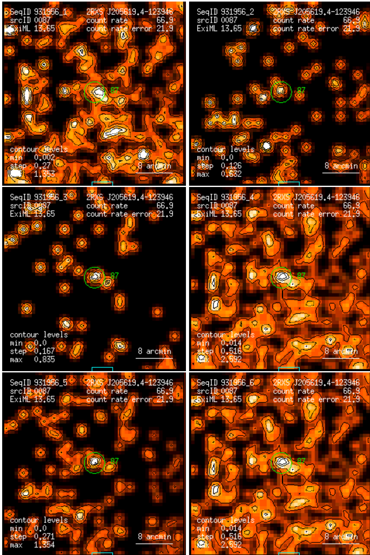
Figure 87: RASS 931956: detection 0087: band rate images, Gaussian filter: (1) PSPC channels 11 – 41, (2) 52 – 90, (3) 91 – 201, (4) 11 – 235, (5) 52 – 201, (6) 11 – 201. Broad band rates in counts/ks. Band rate contour levels in counts/ks/arcmin 2 .
