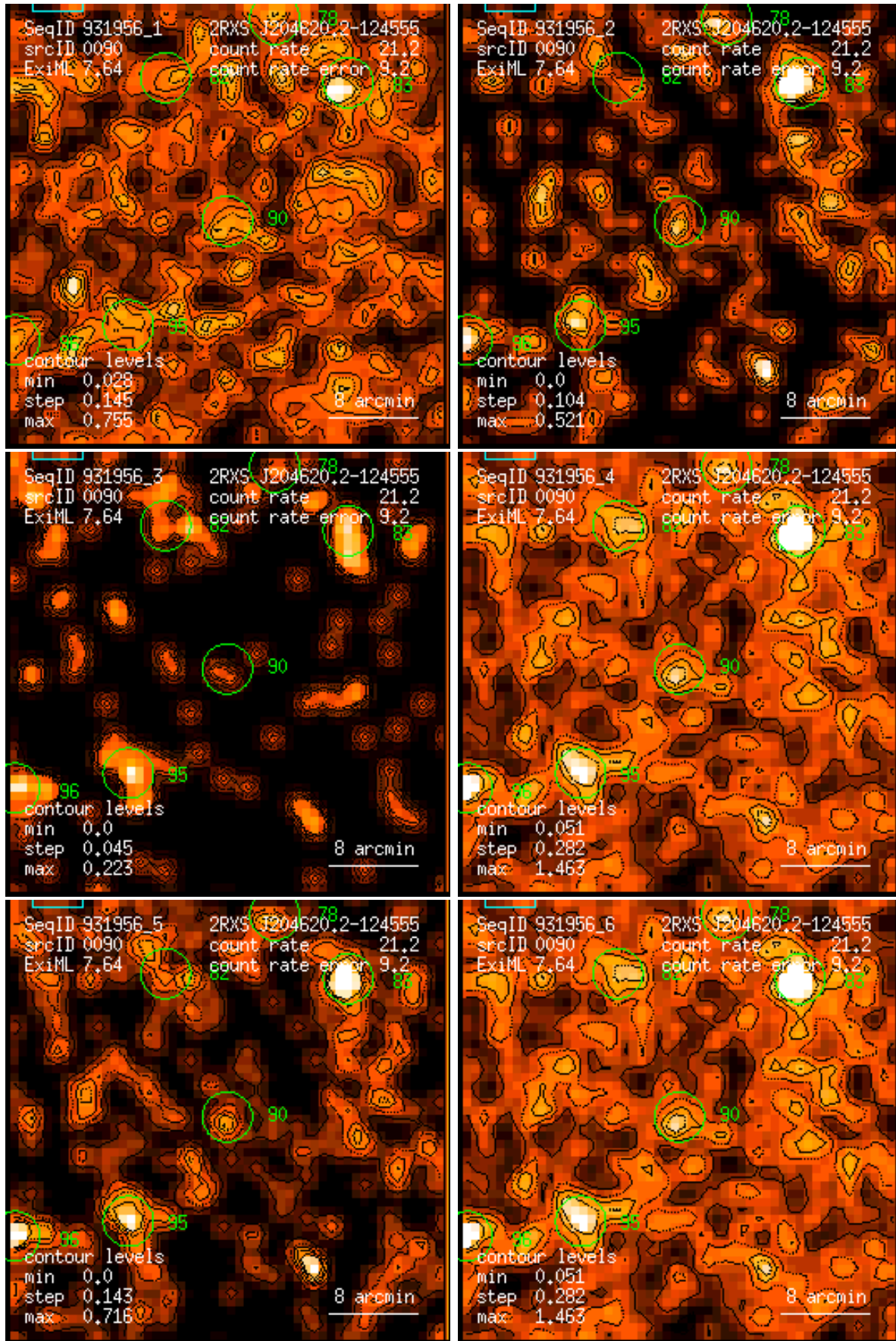
Figure 90: RASS 931956: detection 0090: band rate images, Gaussian filter: (1) PSPC channels 11 – 41, (2) 52 – 90, (3) 91 – 201, (4) 11 – 235, (5) 52 – 201, (6) 11 – 201. Broad band rates in counts/ks. Band rate contour levels in counts/ks/arcmin 2 .
