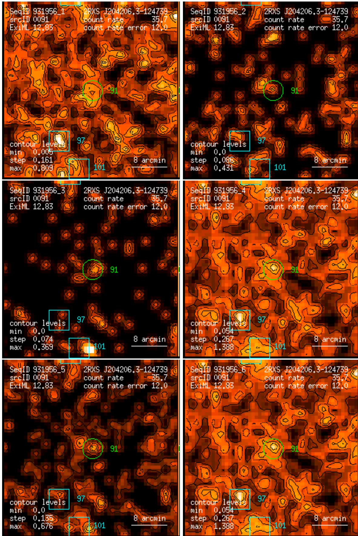
Figure 91: RASS 931956: detection 0091: band rate images, Gaussian filter: (1) PSPC channels 11 – 41, (2) 52 – 90, (3) 91 – 201, (4) 11 – 235, (5) 52 – 201, (6) 11 – 201. Broad band rates in counts/ks. Band rate contour levels in counts/ks/arcmin 2 .
