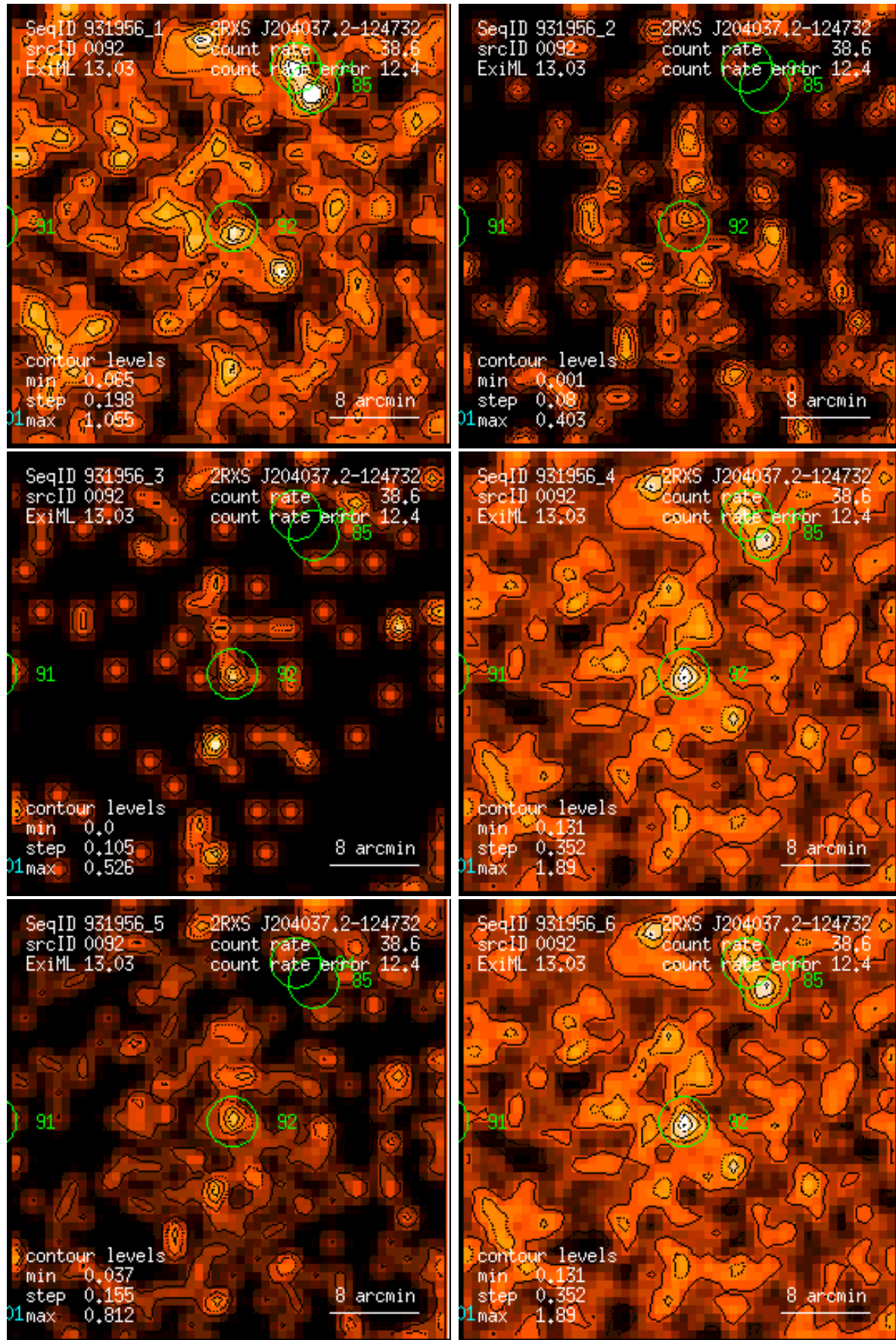
Figure 92: RASS 931956: detection 0092: band rate images, Gaussian filter: (1) PSPC channels 11 – 41, (2) 52 – 90, (3) 91 – 201, (4) 11 – 235, (5) 52 – 201, (6) 11 – 201. Broad band rates in counts/ks. Band rate contour levels in counts/ks/arcmin 2 .
