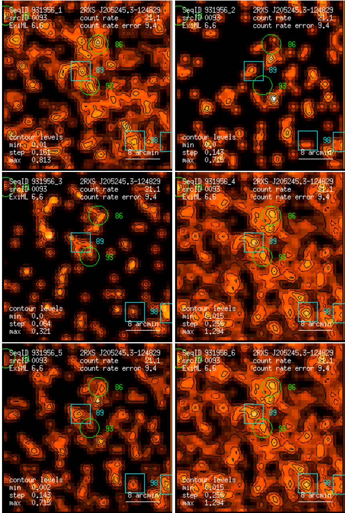
Figure 93: RASS 931956: detection 0093: band rate images, Gaussian filter: (1) PSPC channels 11 – 41, (2) 52 – 90, (3) 91 – 201, (4) 11 – 235, (5) 52 – 201, (6) 11 – 201. Broad band rates in counts/ks. Band rate contour levels in counts/ks/arcmin 2 .
