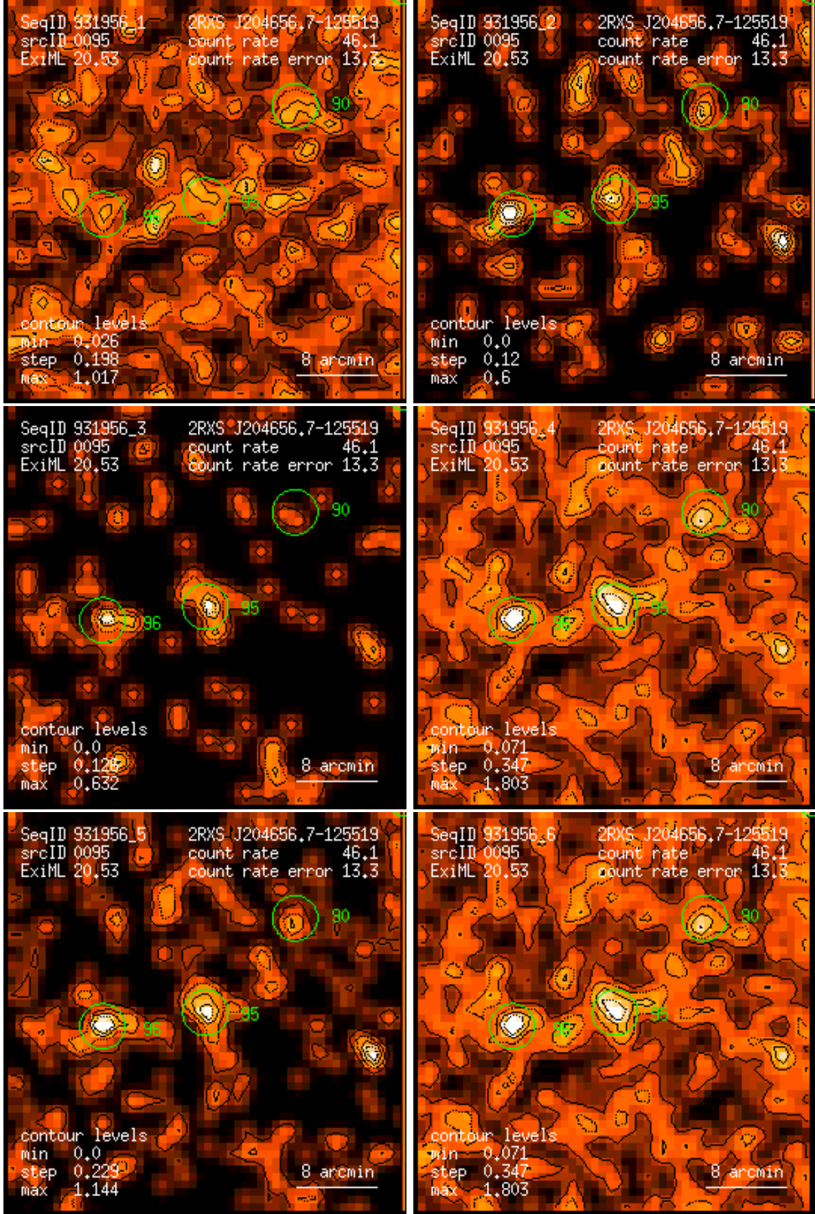
Figure 95: RASS 931956: detection 0095: band rate images, Gaussian filter: (1) PSPC channels 11 – 41, (2) 52 – 90, (3) 91 – 201, (4) 11 – 235, (5) 52 – 201, (6) 11 – 201. Broad band rates in counts/ks. Band rate contour levels in counts/ks/arcmin 2 .
