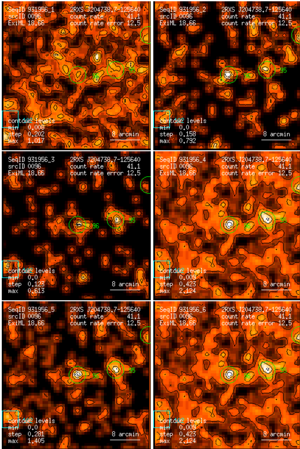
Figure 96: RASS 931956: detection 0096: band rate images, Gaussian filter: (1) PSPC channels 11 – 41, (2) 52 – 90, (3) 91 – 201, (4) 11 – 235, (5) 52 – 201, (6) 11 – 201. Broad band rates in counts/ks. Band rate contour levels in counts/ks/arcmin 2 .
