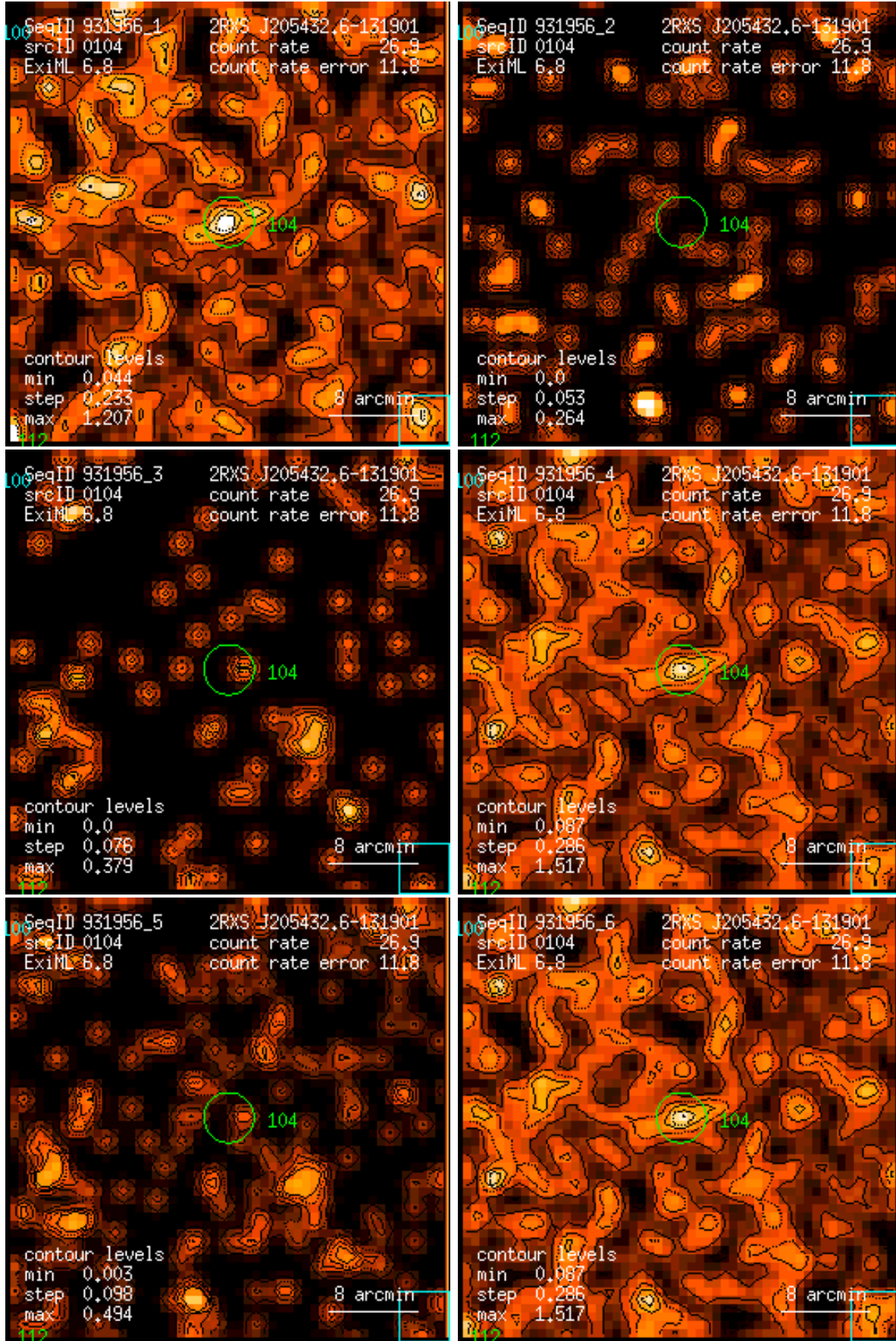
Figure 104: RASS 931956: detection 0104: band rate images, Gaussian filter: (1) PSPC channels 11 – 41, (2) 52 – 90, (3) 91 – 201, (4) 11 – 235, (5) 52 – 201, (6) 11 – 201. Broad band rates in counts/ks. Band rate contour levels in counts/ks/arcmin 2 .
