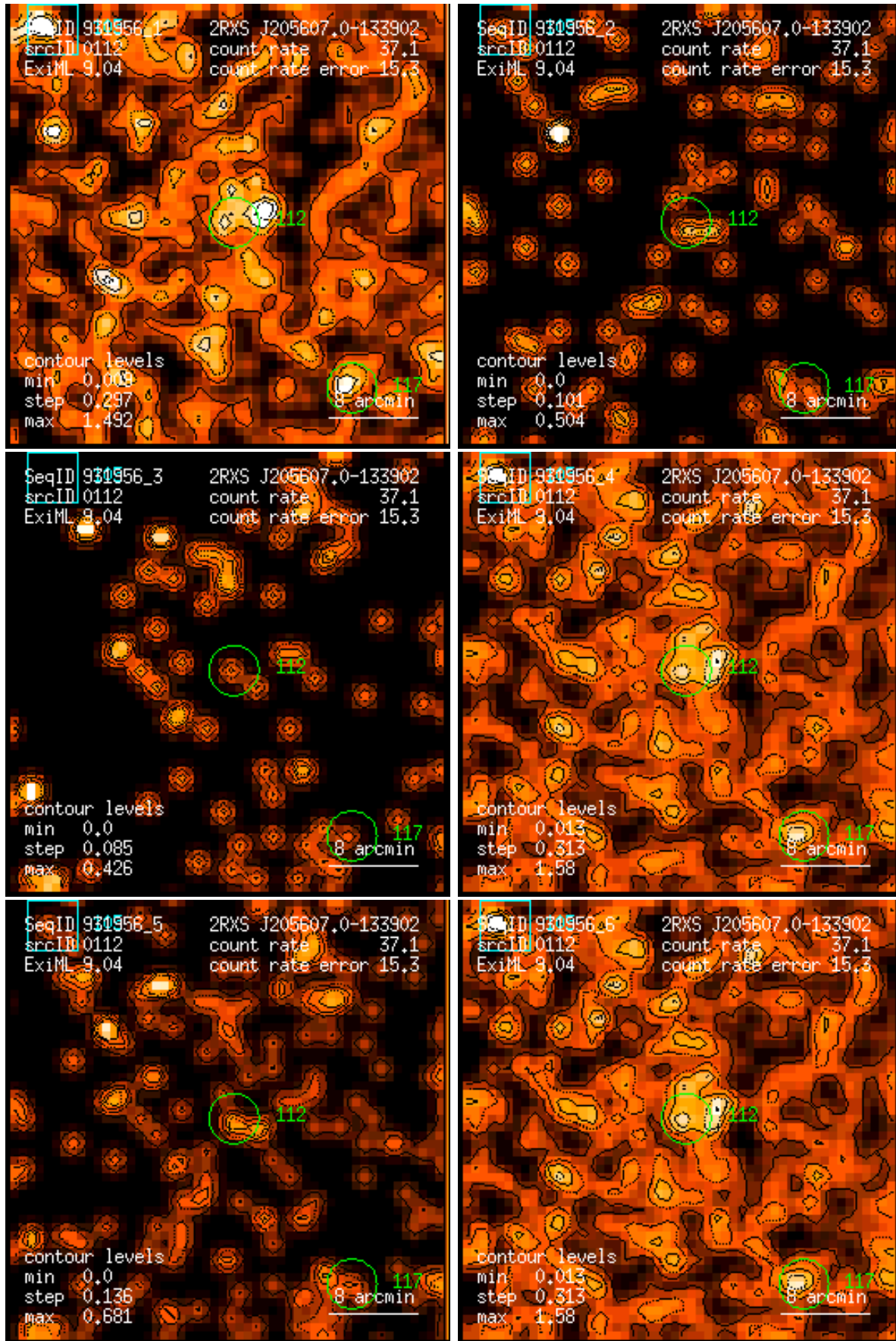
Figure 112: RASS 931956: detection 0112: band rate images, Gaussian filter: (1) PSPC channels 11 – 41, (2) 52 – 90, (3) 91 – 201, (4) 11 – 235, (5) 52 – 201, (6) 11 – 201. Broad band rates in counts/ks. Band rate contour levels in counts/ks/arcmin 2 .
