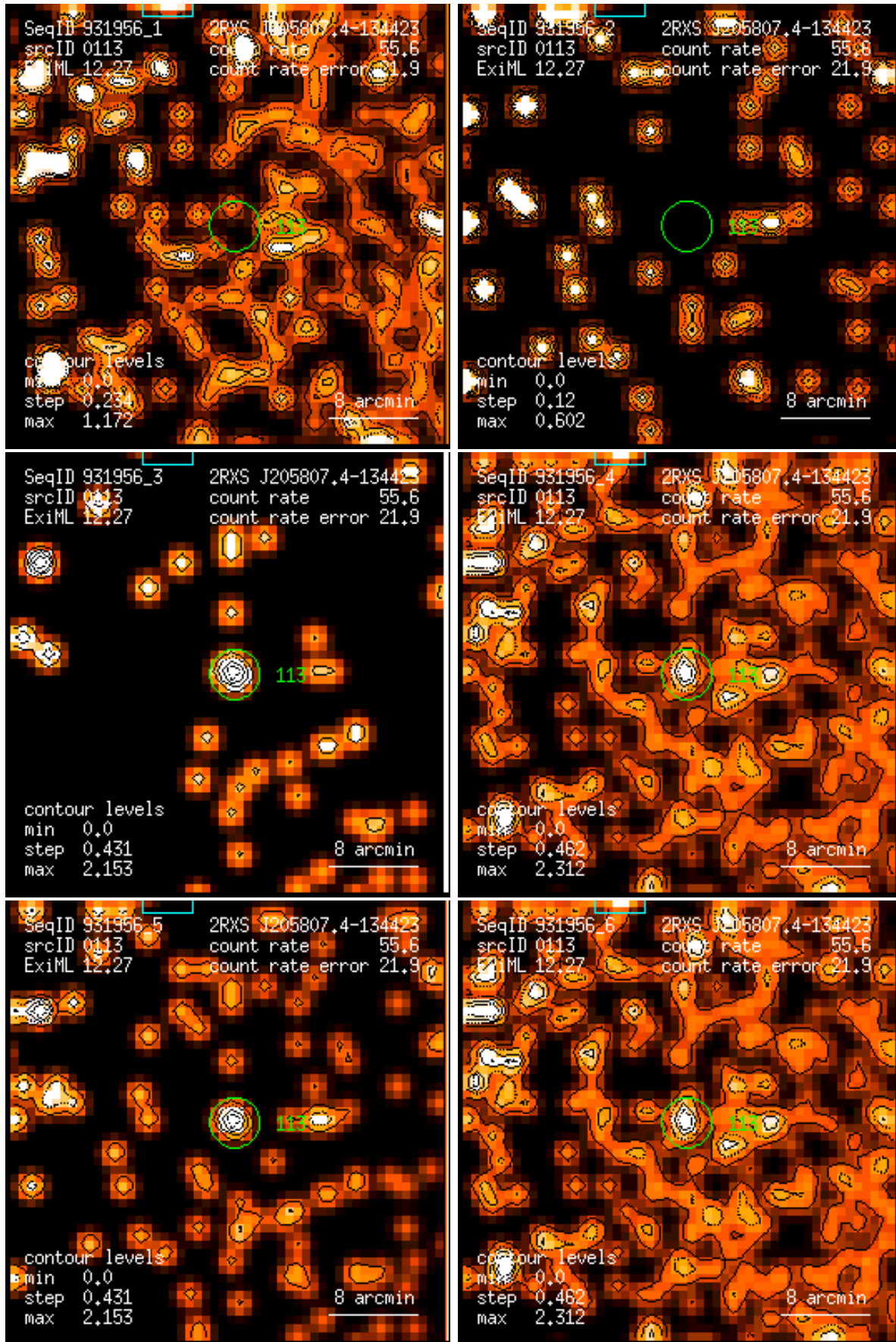
Figure 113: RASS 931956: detection 0113: band rate images, Gaussian filter: (1) PSPC channels 11 – 41, (2) 52 – 90, (3) 91 – 201, (4) 11 – 235, (5) 52 – 201, (6) 11 – 201. Broad band rates in counts/ks. Band rate contour levels in counts/ks/arcmin 2 .
