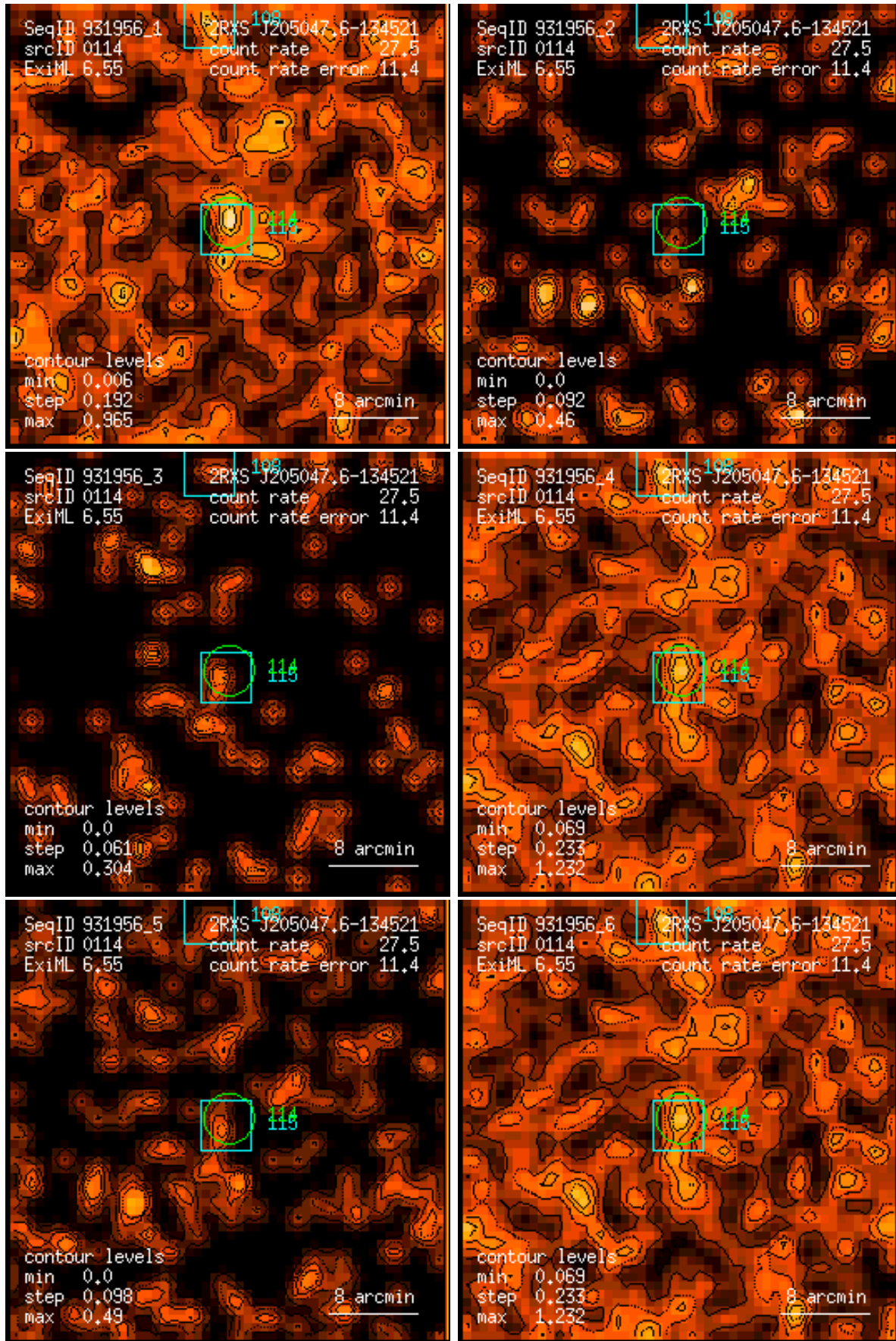
Figure 114: RASS 931956: detection 0114: band rate images, Gaussian filter: (1) PSPC channels 11 – 41, (2) 52 – 90, (3) 91 – 201, (4) 11 – 235, (5) 52 – 201, (6) 11 – 201. Broad band rates in counts/ks. Band rate contour levels in counts/ks/arcmin 2 .
