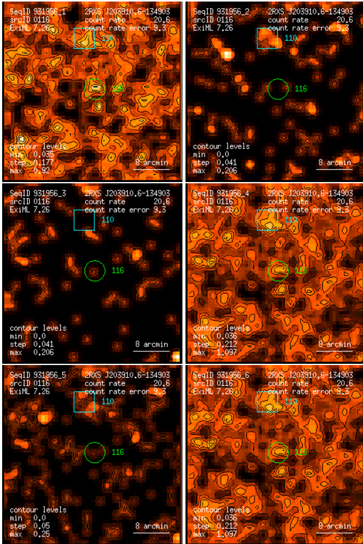
Figure 116: RASS 931956: detection 0116: band rate images, Gaussian filter: (1) PSPC channels 11 – 41, (2) 52 – 90, (3) 91 – 201, (4) 11 – 235, (5) 52 – 201, (6) 11 – 201. Broad band rates in counts/ks. Band rate contour levels in counts/ks/arcmin 2 .
