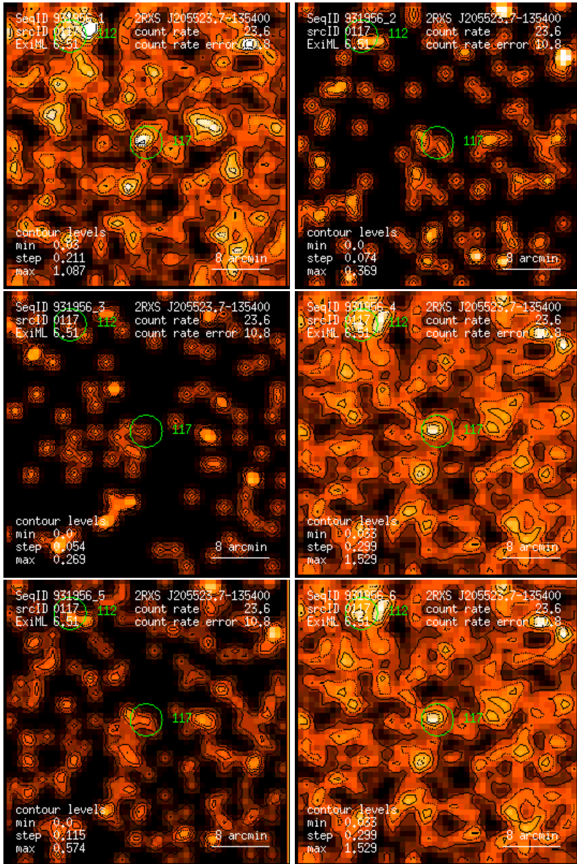
Figure 117: RASS 931956: detection 0117: band rate images, Gaussian filter: (1) PSPC channels 11 – 41, (2) 52 – 90, (3) 91 – 201, (4) 11 – 235, (5) 52 – 201, (6) 11 – 201. Broad band rates in counts/ks. Band rate contour levels in counts/ks/arcmin 2 .
