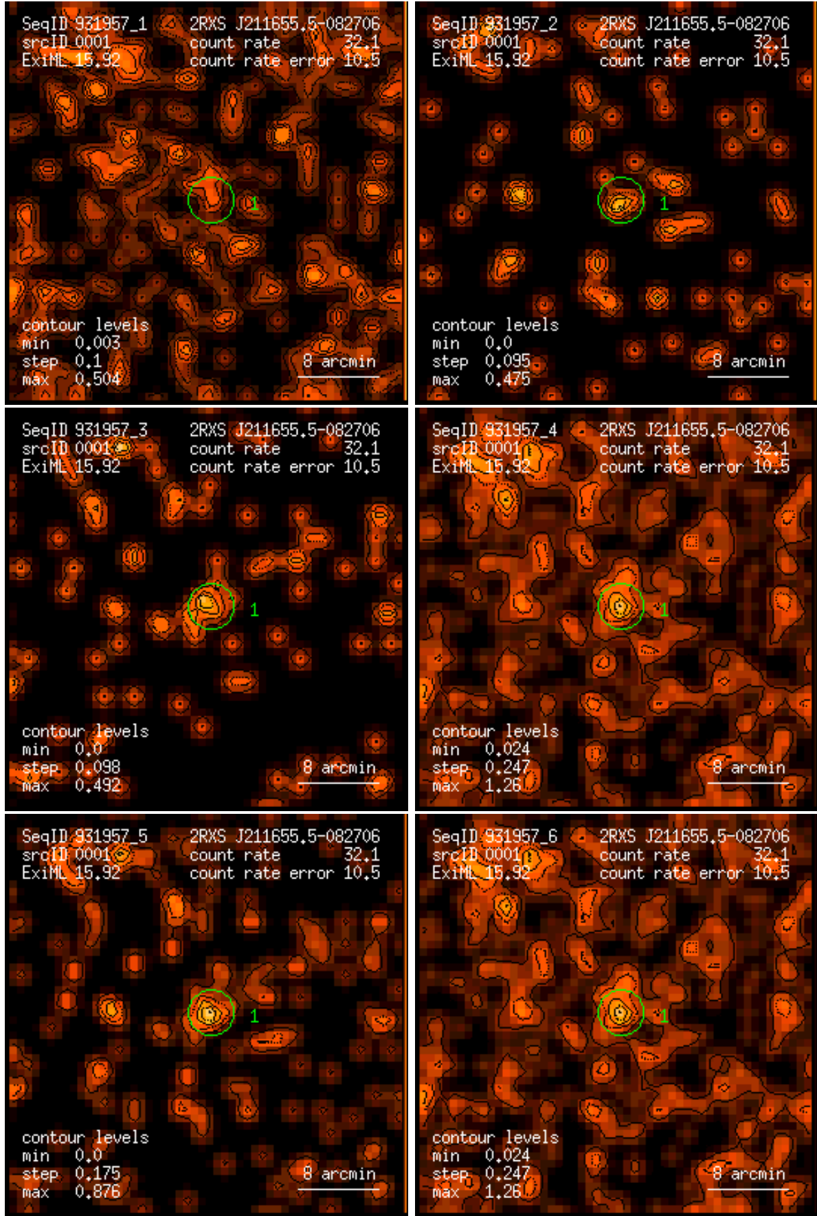
Figure 1: RASS 931957: detection 0001: band rate images, Gaussian filter: (1) PSPC channels 11 – 41, (2) 52 – 90, (3) 91 – 201, (4) 11 – 235, (5) 52 – 201, (6) 11 – 201. Broad band rates in counts/ks. Band rate contour levels in counts/ks/arcmin 2 .
