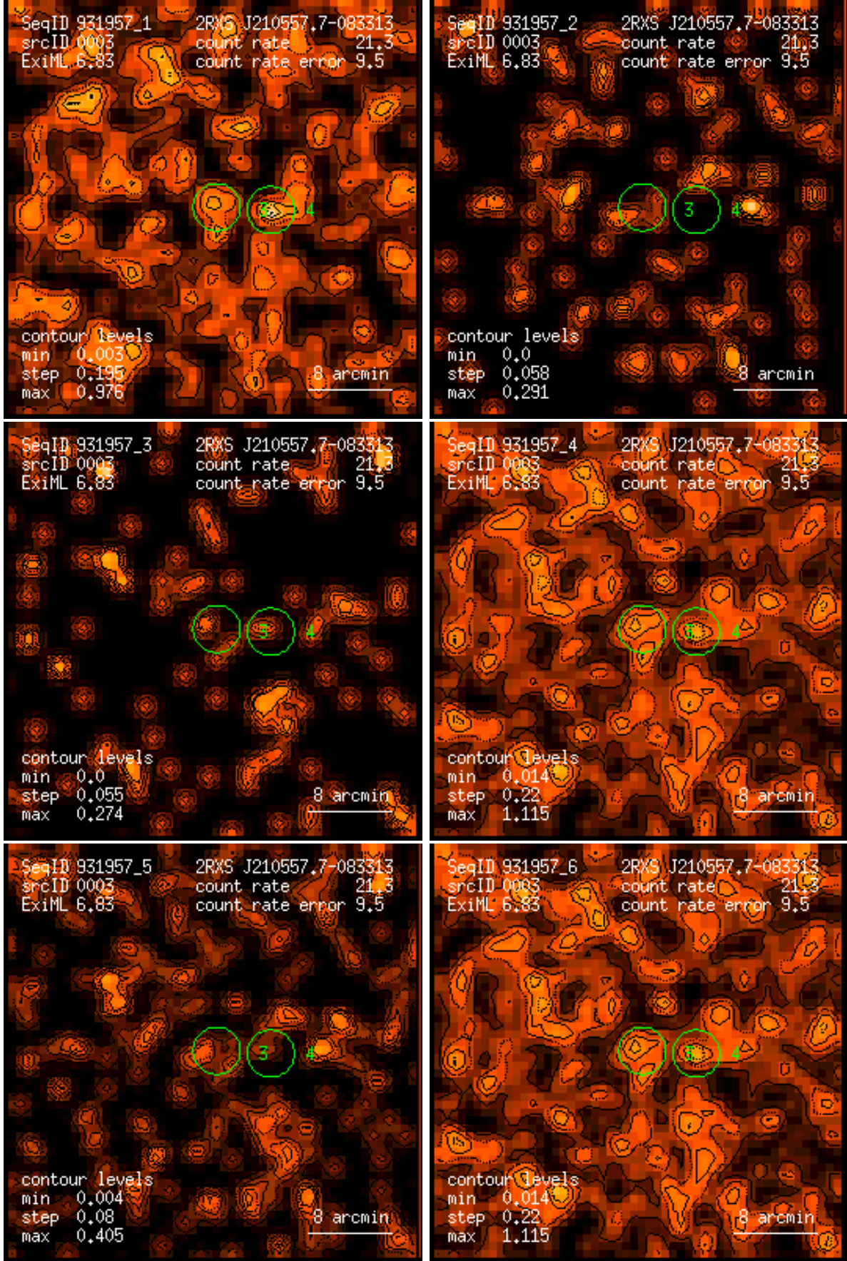
Figure 3: RASS 931957: detection 0003: band rate images, Gaussian filter: (1) PSPC channels 11 – 41, (2) 52 – 90, (3) 91 – 201, (4) 11 – 235, (5) 52 – 201, (6) 11 – 201. Broad band rates in counts/ks. Band rate contour levels in counts/ks/arcmin 2 .
