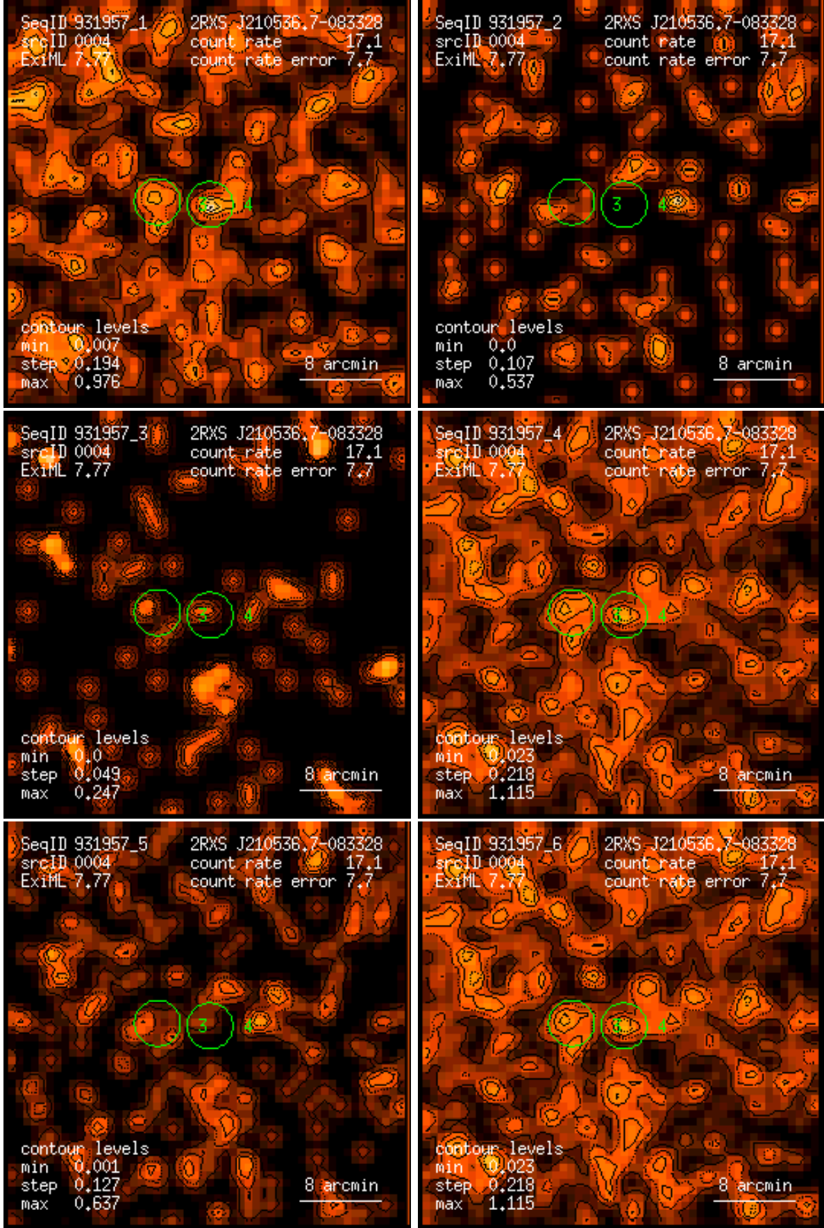
Figure 4: RASS 931957: detection 0004: band rate images, Gaussian filter: (1) PSPC channels 11 – 41, (2) 52 – 90, (3) 91 – 201, (4) 11 – 235, (5) 52 – 201, (6) 11 – 201. Broad band rates in counts/ks. Band rate contour levels in counts/ks/arcmin 2 .
