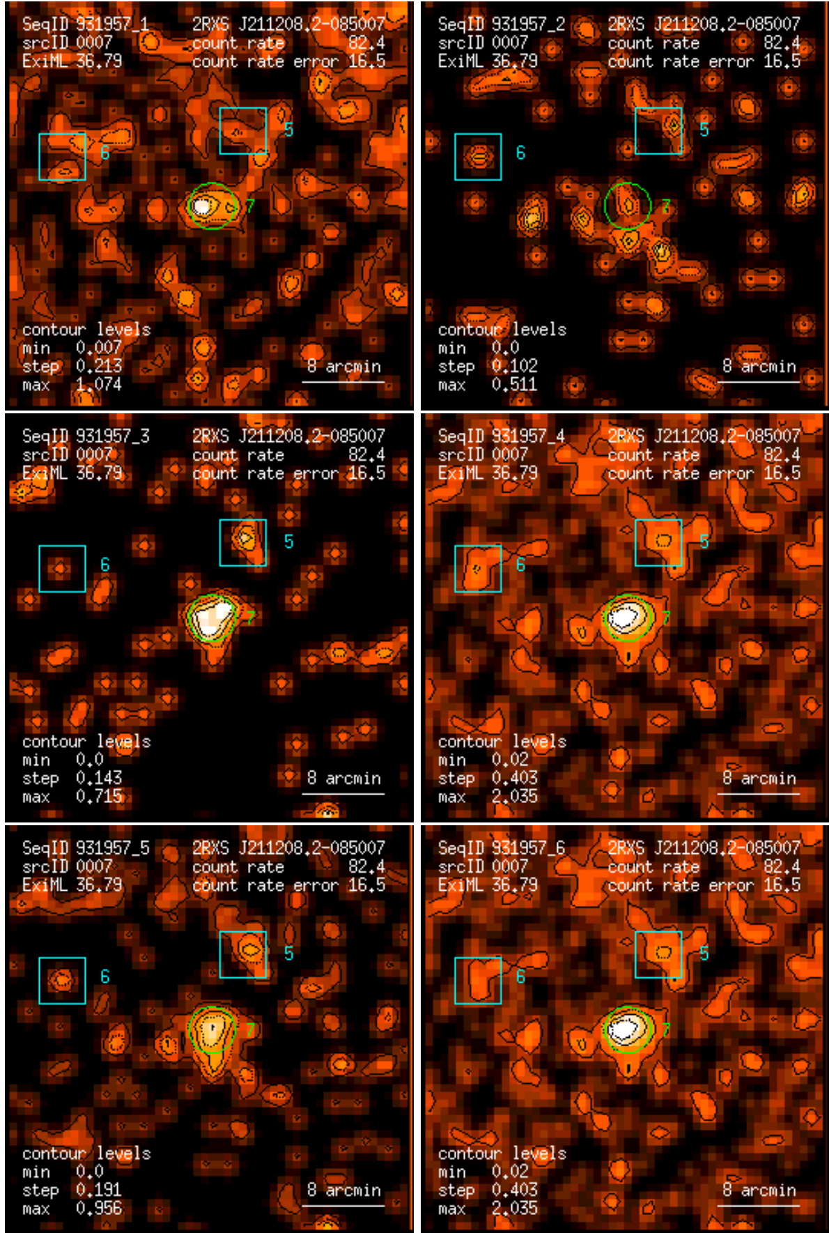
Figure 7: RASS 931957: detection 0007: band rate images, Gaussian filter: (1) PSPC channels 11 – 41, (2) 52 – 90, (3) 91 – 201, (4) 11 – 235, (5) 52 – 201, (6) 11 – 201. Broad band rates in counts/ks. Band rate contour levels in counts/ks/arcmin 2 .
