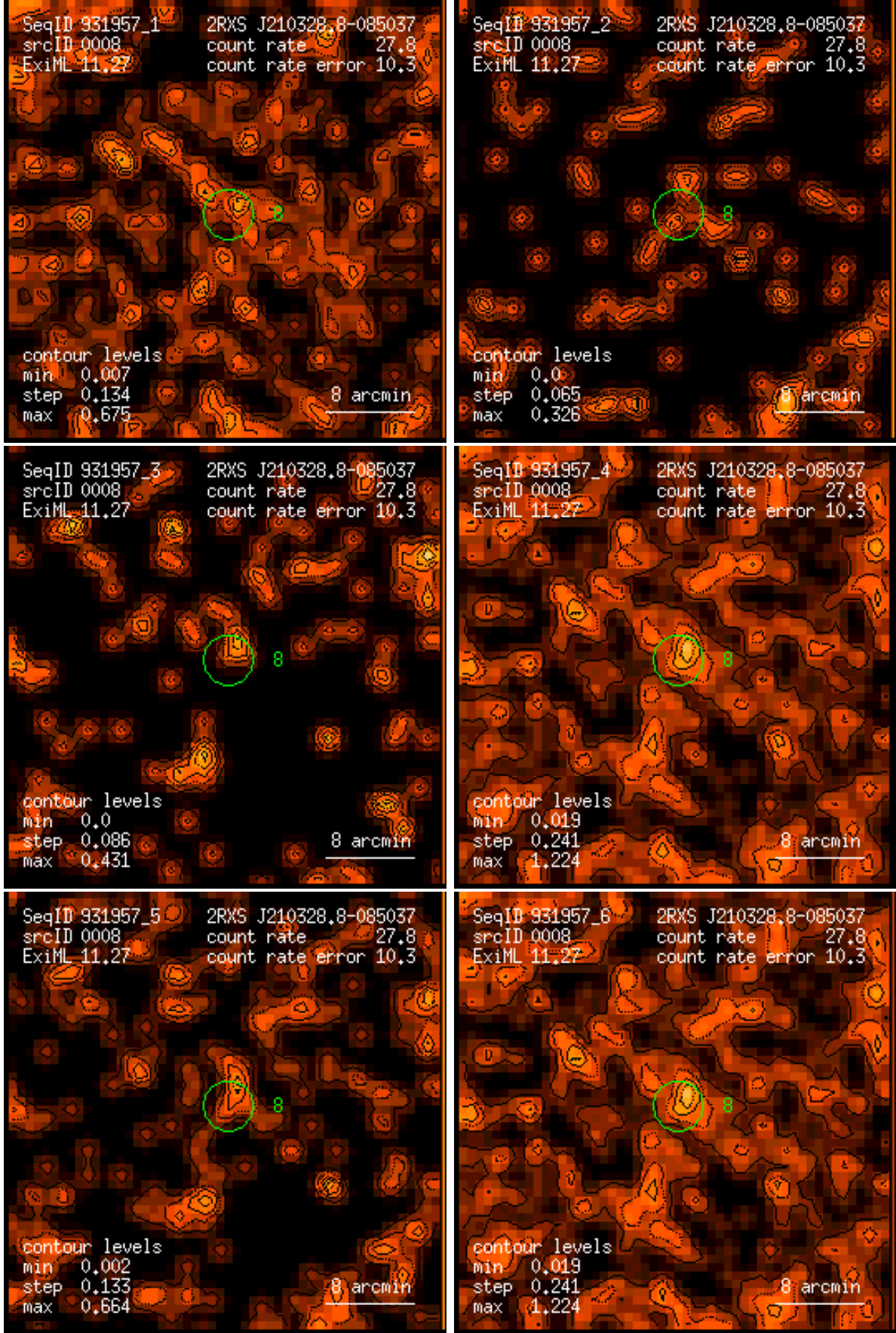
Figure 8: RASS 931957: detection 0008: band rate images, Gaussian filter: (1) PSPC channels 11 – 41, (2) 52 – 90, (3) 91 – 201, (4) 11 – 235, (5) 52 – 201, (6) 11 – 201. Broad band rates in counts/ks. Band rate contour levels in counts/ks/arcmin 2 .
