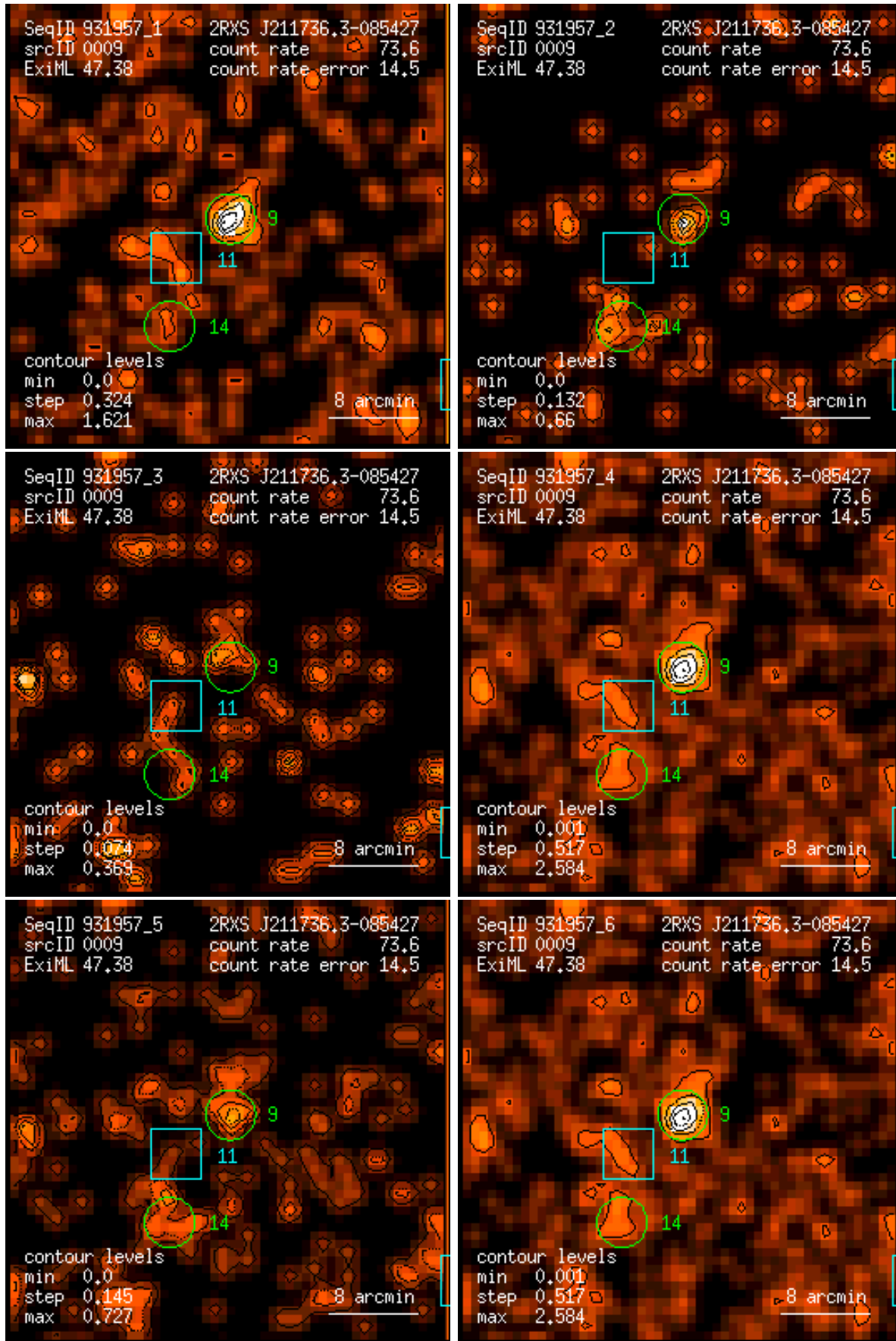
Figure 9: RASS 931957: detection 0009: band rate images, Gaussian filter: (1) PSPC channels 11 – 41, (2) 52 – 90, (3) 91 – 201, (4) 11 – 235, (5) 52 – 201, (6) 11 – 201. Broad band rates in counts/ks. Band rate contour levels in counts/ks/arcmin 2 .
