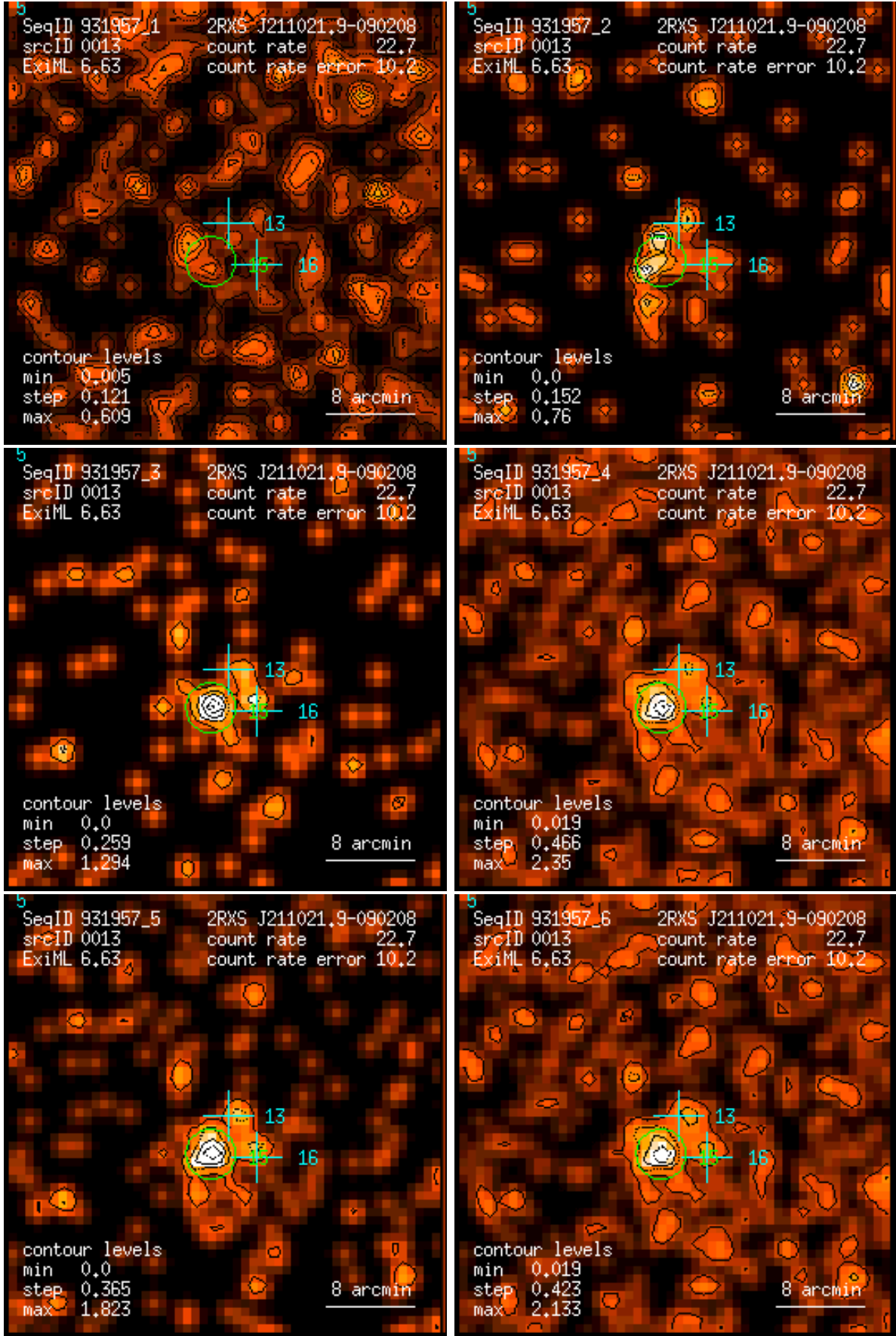
Figure 13: RASS 931957: detection 0013: band rate images, Gaussian filter: (1) PSPC channels 11 – 41, (2) 52 – 90, (3) 91 – 201, (4) 11 – 235, (5) 52 – 201, (6) 11 – 201. Broad band rates in counts/ks. Band rate contour levels in counts/ks/arcmin 2 .
