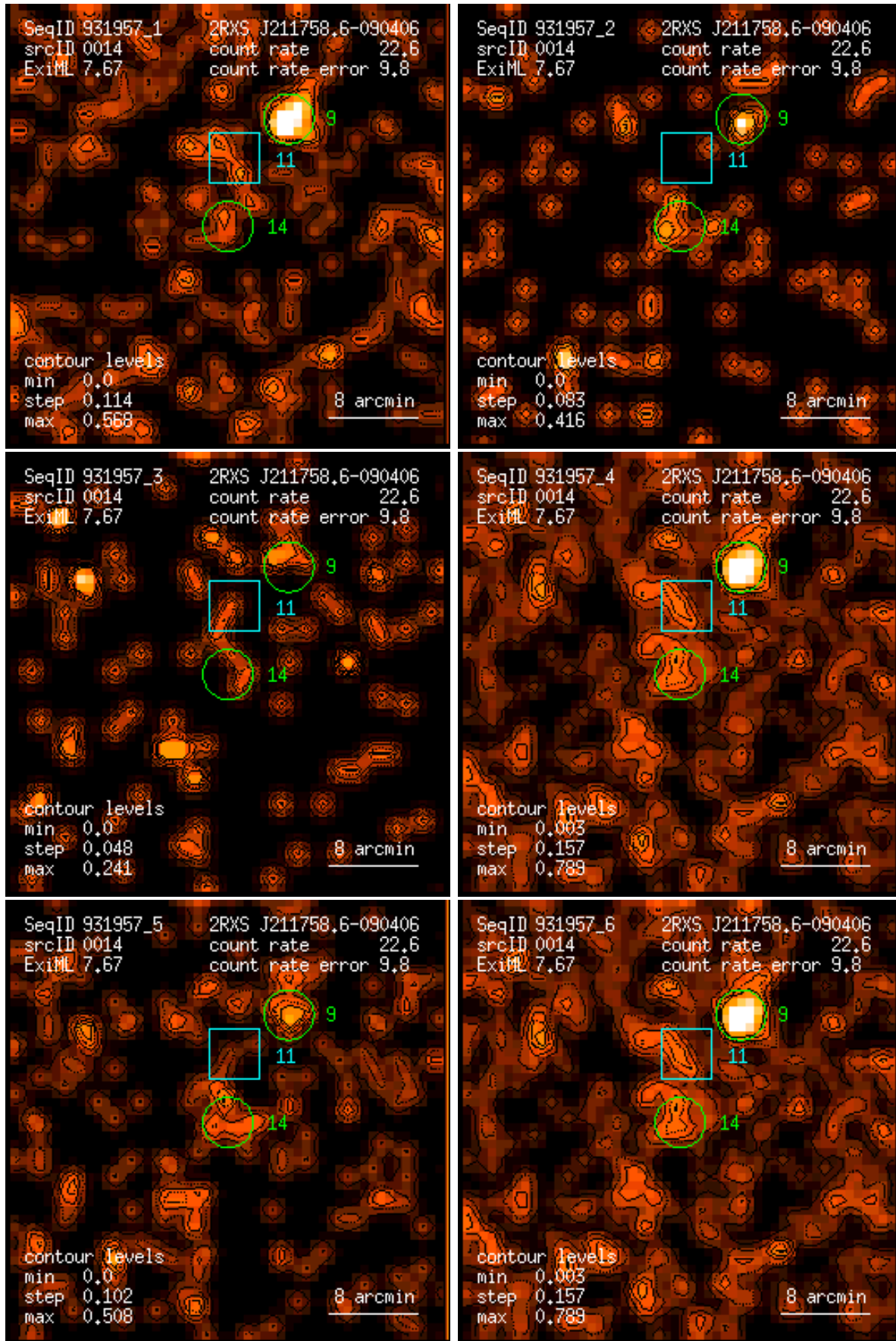
Figure 14: RASS 931957: detection 0014: band rate images, Gaussian filter: (1) PSPC channels 11 – 41, (2) 52 – 90, (3) 91 – 201, (4) 11 – 235, (5) 52 – 201, (6) 11 – 201. Broad band rates in counts/ks. Band rate contour levels in counts/ks/arcmin 2 .
