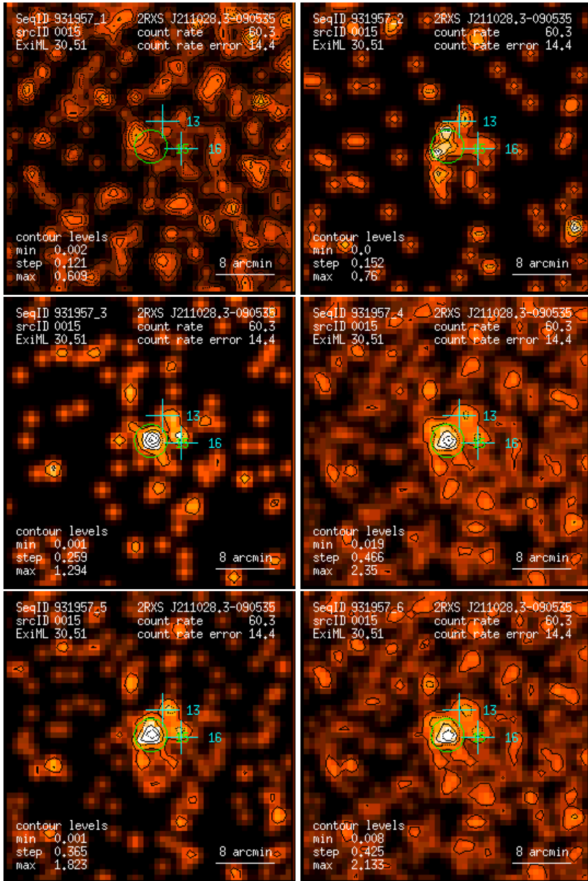
Figure 15: RASS 931957: detection 0015: band rate images, Gaussian filter: (1) PSPC channels 11 – 41, (2) 52 – 90, (3) 91 – 201, (4) 11 – 235, (5) 52 – 201, (6) 11 – 201. Broad band rates in counts/ks. Band rate contour levels in counts/ks/arcmin 2 .
