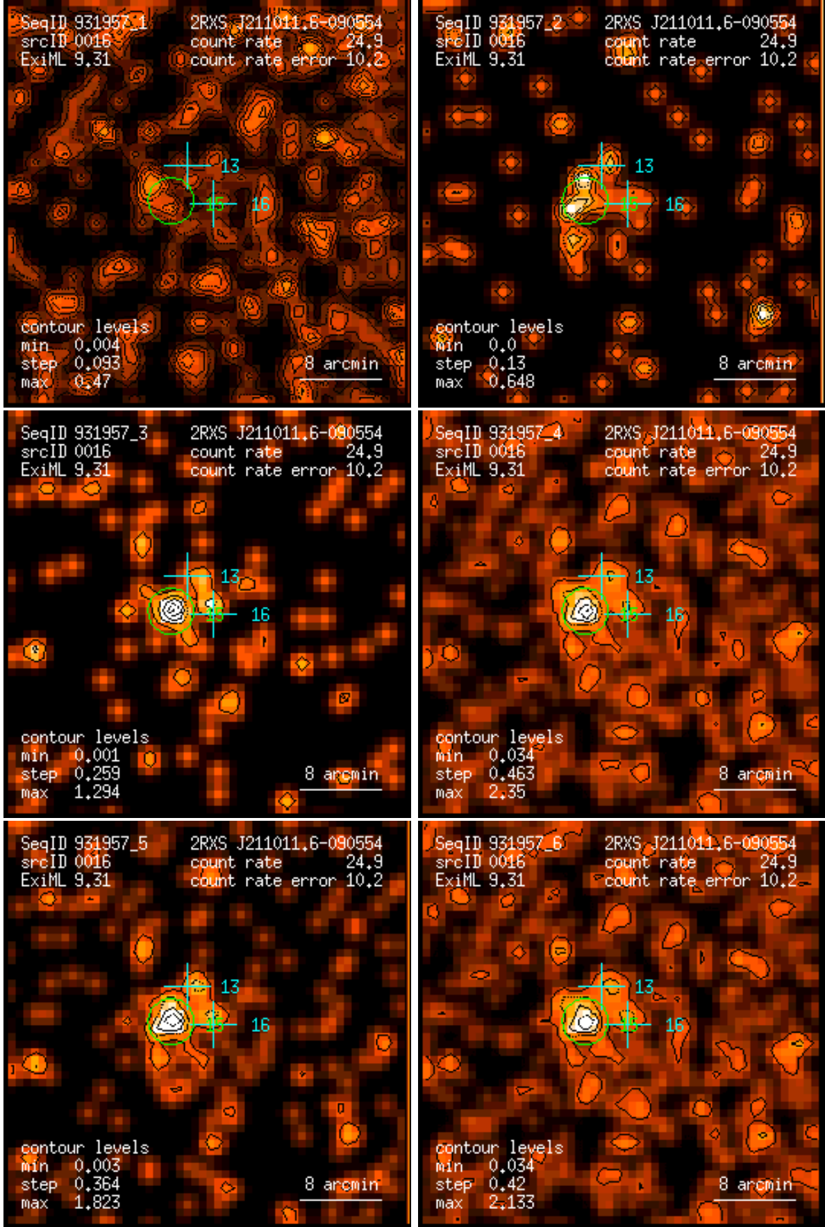
Figure 16: RASS 931957: detection 0016: band rate images, Gaussian filter: (1) PSPC channels 11 – 41, (2) 52 – 90, (3) 91 – 201, (4) 11 – 235, (5) 52 – 201, (6) 11 – 201. Broad band rates in counts/ks. Band rate contour levels in counts/ks/arcmin 2 .
