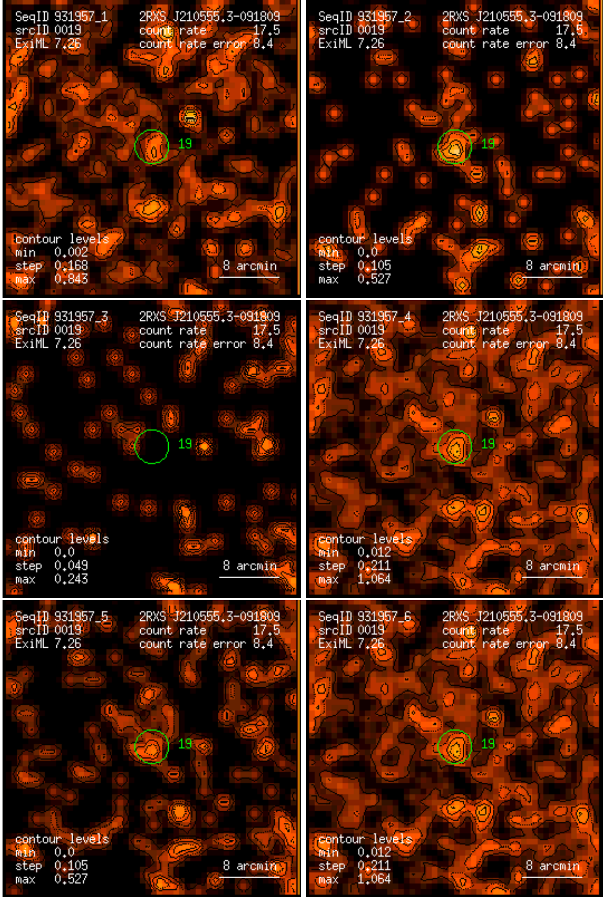
Figure 19: RASS 931957: detection 0019: band rate images, Gaussian filter: (1) PSPC channels 11 – 41, (2) 52 – 90, (3) 91 – 201, (4) 11 – 235, (5) 52 – 201, (6) 11 – 201. Broad band rates in counts/ks. Band rate contour levels in counts/ks/arcmin 2 .
