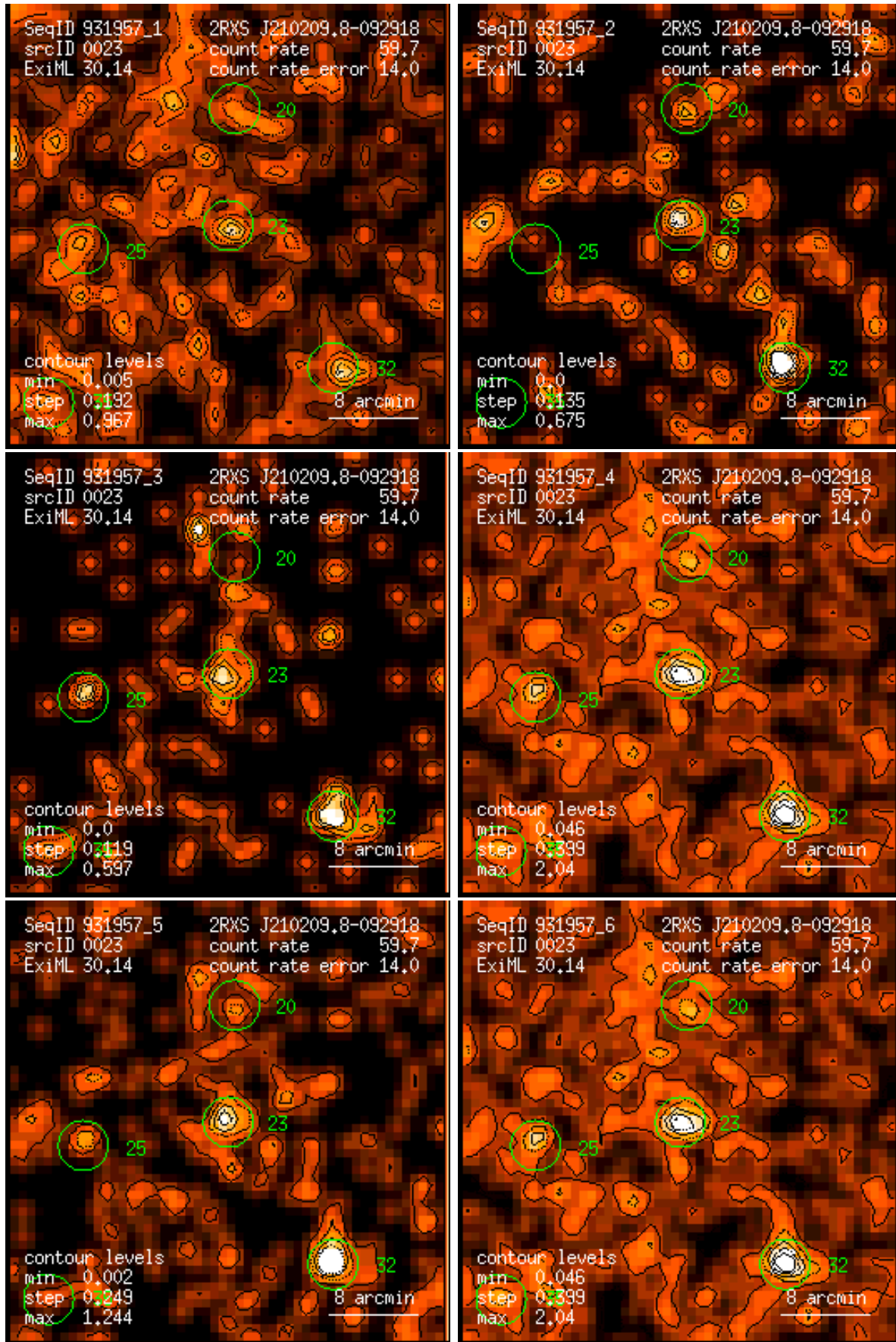
Figure 23: RASS 931957: detection 0023: band rate images, Gaussian filter: (1) PSPC channels 11 – 41, (2) 52 – 90, (3) 91 – 201, (4) 11 – 235, (5) 52 – 201, (6) 11 – 201. Broad band rates in counts/ks. Band rate contour levels in counts/ks/arcmin 2 .
