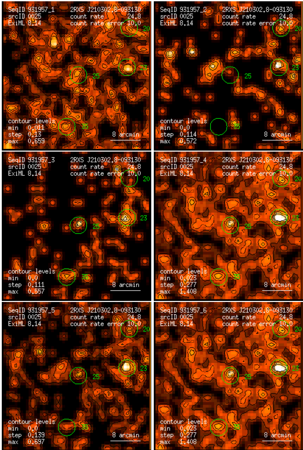
Figure 25: RASS 931957: detection 0025: band rate images, Gaussian filter: (1) PSPC channels 11 – 41, (2) 52 – 90, (3) 91 – 201, (4) 11 – 235, (5) 52 – 201, (6) 11 – 201. Broad band rates in counts/ks. Band rate contour levels in counts/ks/arcmin 2 .
