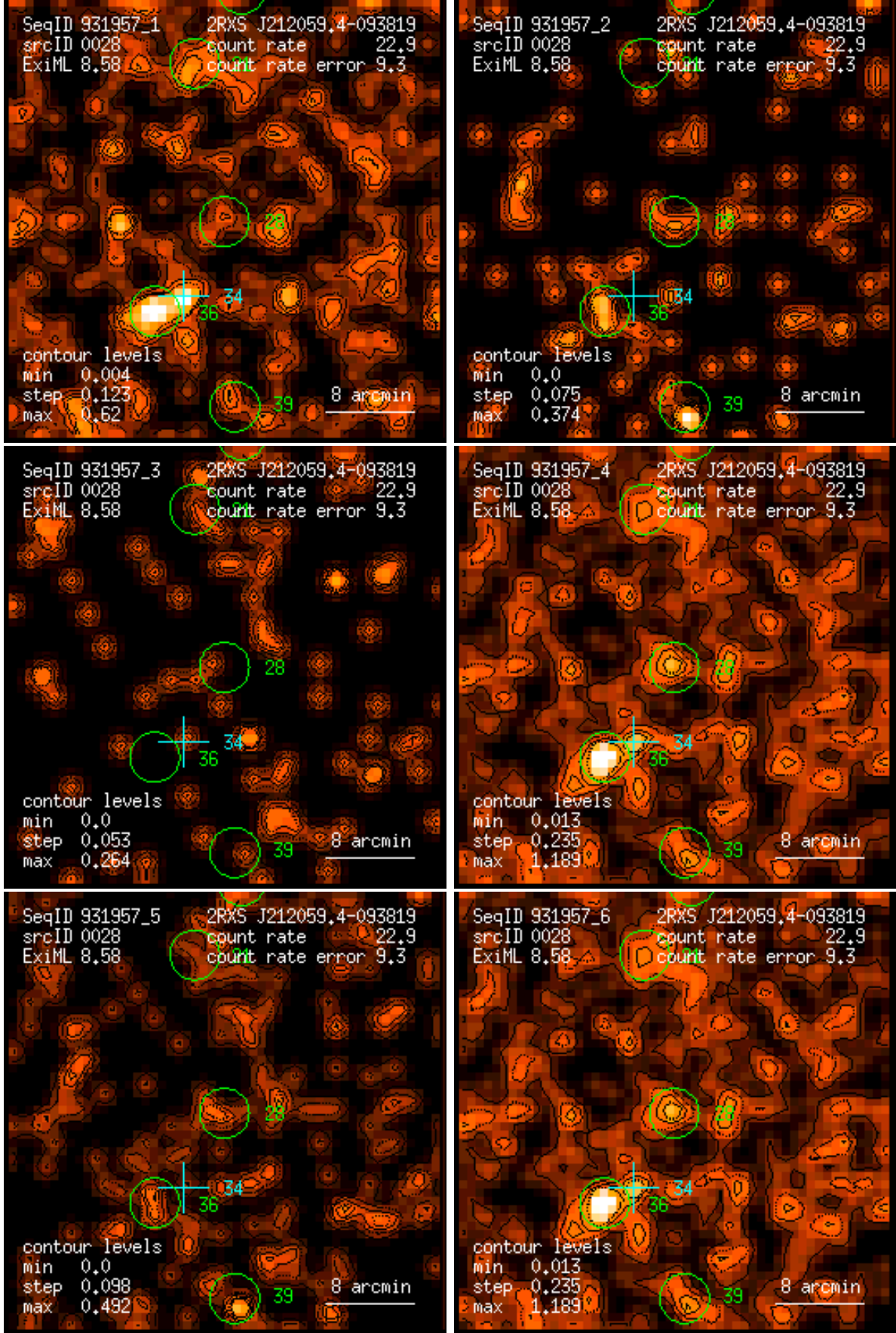
Figure 28: RASS 931957: detection 0028: band rate images, Gaussian filter: (1) PSPC channels 11 – 41, (2) 52 – 90, (3) 91 – 201, (4) 11 – 235, (5) 52 – 201, (6) 11 – 201. Broad band rates in counts/ks. Band rate contour levels in counts/ks/arcmin 2 .
