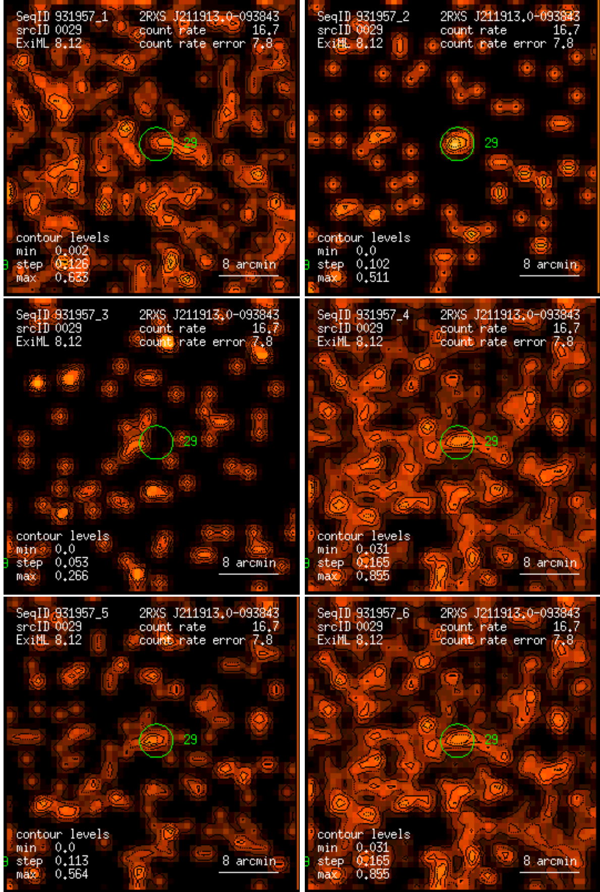
Figure 29: RASS 931957: detection 0029: band rate images, Gaussian filter: (1) PSPC channels 11 – 41, (2) 52 – 90, (3) 91 – 201, (4) 11 – 235, (5) 52 – 201, (6) 11 – 201. Broad band rates in counts/ks. Band rate contour levels in counts/ks/arcmin 2 .
