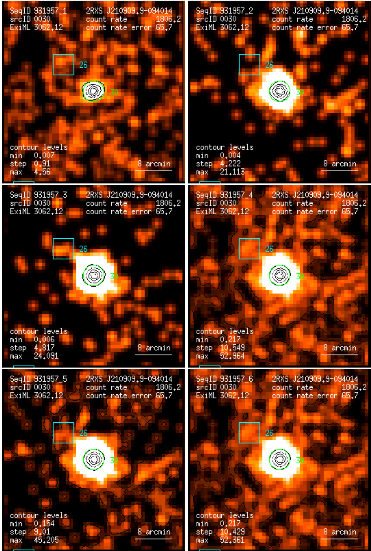
Figure 30: RASS 931957: detection 0030: band rate images, Gaussian filter: (1) PSPC channels 11 – 41, (2) 52 – 90, (3) 91 – 201, (4) 11 – 235, (5) 52 – 201, (6) 11 – 201. Broad band rates in counts/ks. Band rate contour levels in counts/ks/arcmin 2 .
