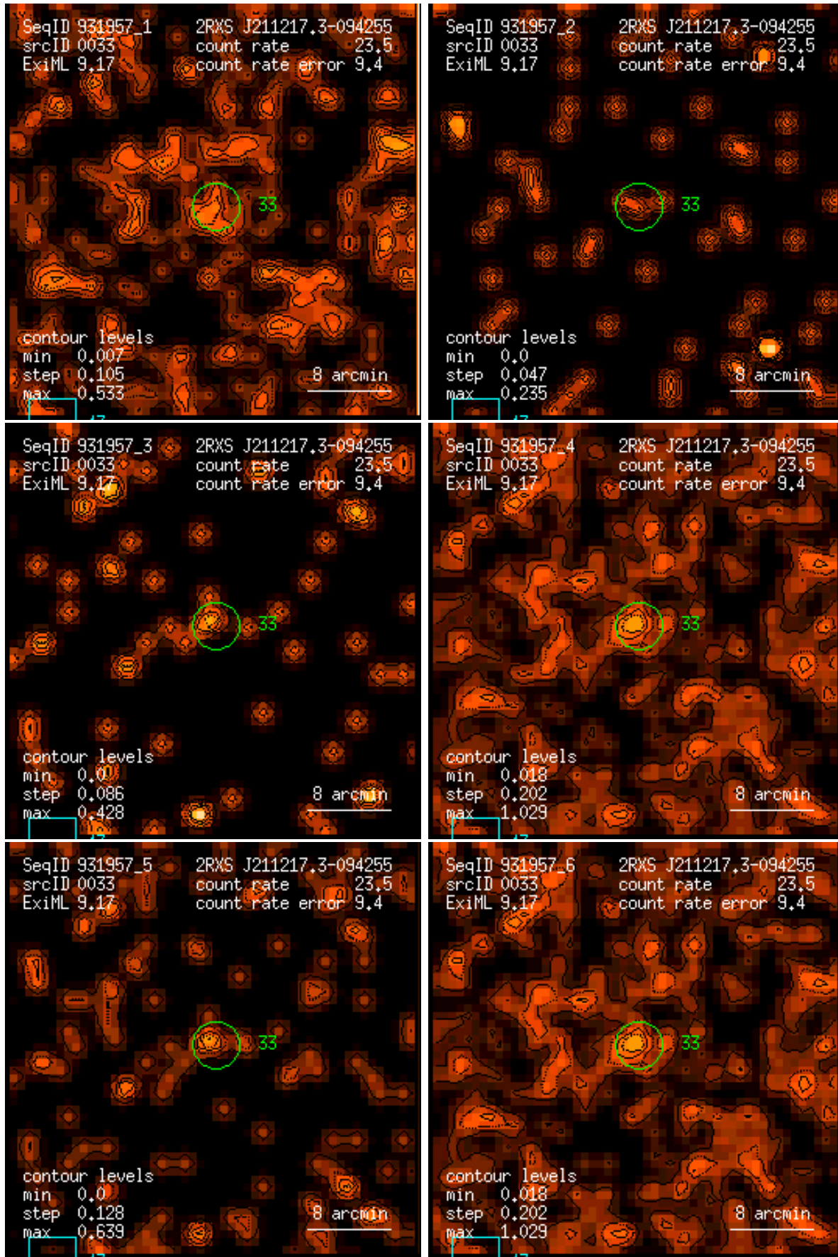
Figure 33: RASS 931957: detection 0033: band rate images, Gaussian filter: (1) PSPC channels 11 – 41, (2) 52 – 90, (3) 91 – 201, (4) 11 – 235, (5) 52 – 201, (6) 11 – 201. Broad band rates in counts/ks. Band rate contour levels in counts/ks/arcmin 2 .
