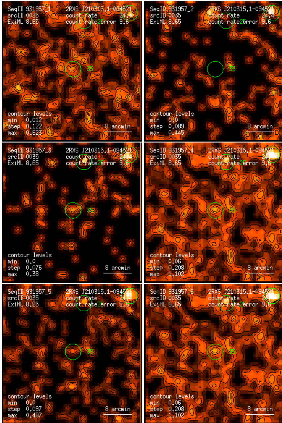
Figure 35: RASS 931957: detection 0035: band rate images, Gaussian filter: (1) PSPC channels 11 – 41, (2) 52 – 90, (3) 91 – 201, (4) 11 – 235, (5) 52 – 201, (6) 11 – 201. Broad band rates in counts/ks. Band rate contour levels in counts/ks/arcmin 2 .
