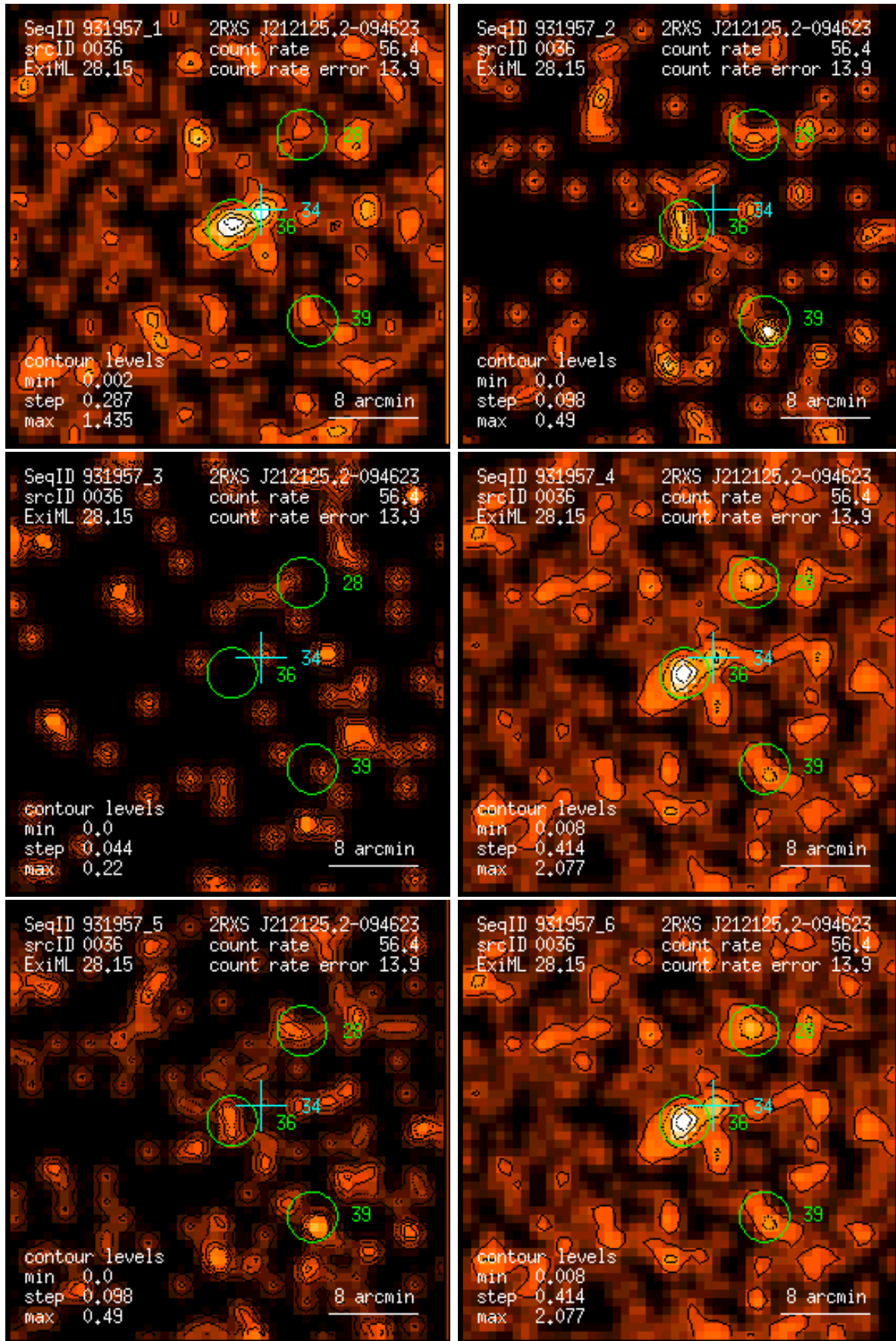
Figure 36: RASS 931957: detection 0036: band rate images, Gaussian filter: (1) PSPC channels 11 – 41, (2) 52 – 90, (3) 91 – 201, (4) 11 – 235, (5) 52 – 201, (6) 11 – 201. Broad band rates in counts/ks. Band rate contour levels in counts/ks/arcmin 2 .
