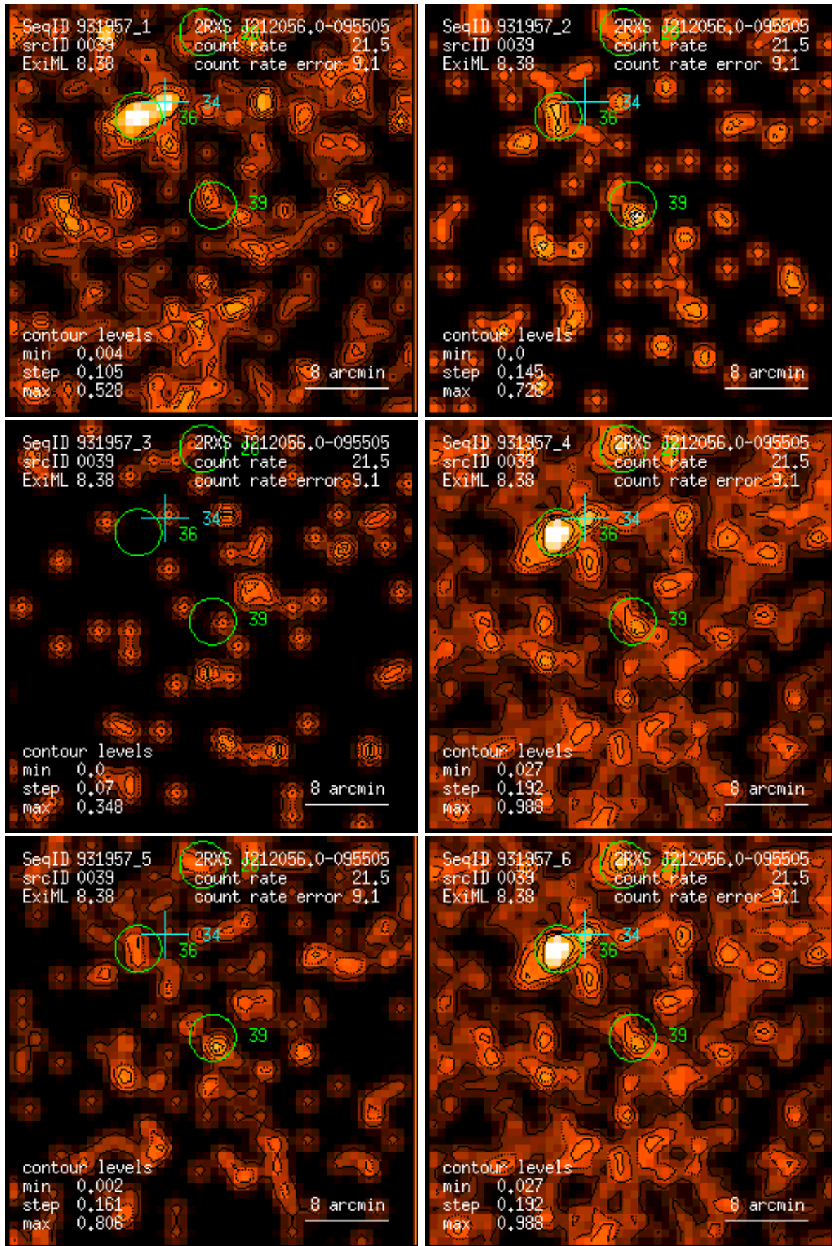
Figure 39: RASS 931957: detection 0039: band rate images, Gaussian filter: (1) PSPC channels 11 – 41, (2) 52 – 90, (3) 91 – 201, (4) 11 – 235, (5) 52 – 201, (6) 11 – 201. Broad band rates in counts/ks. Band rate contour levels in counts/ks/arcmin 2 .
