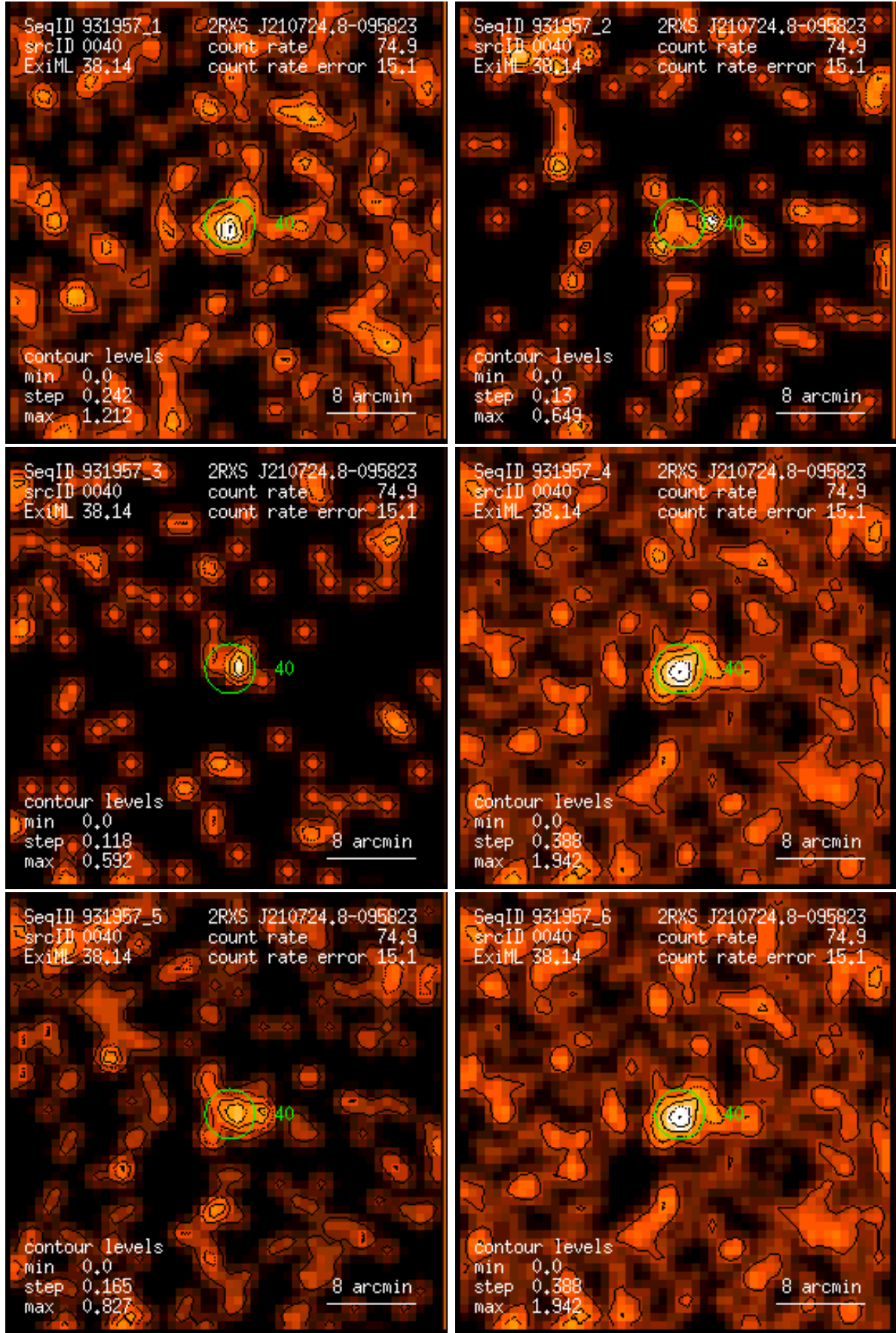
Figure 40: RASS 931957: detection 0040: band rate images, Gaussian filter: (1) PSPC channels 11 – 41, (2) 52 – 90, (3) 91 – 201, (4) 11 – 235, (5) 52 – 201, (6) 11 – 201. Broad band rates in counts/ks. Band rate contour levels in counts/ks/arcmin 2 .
