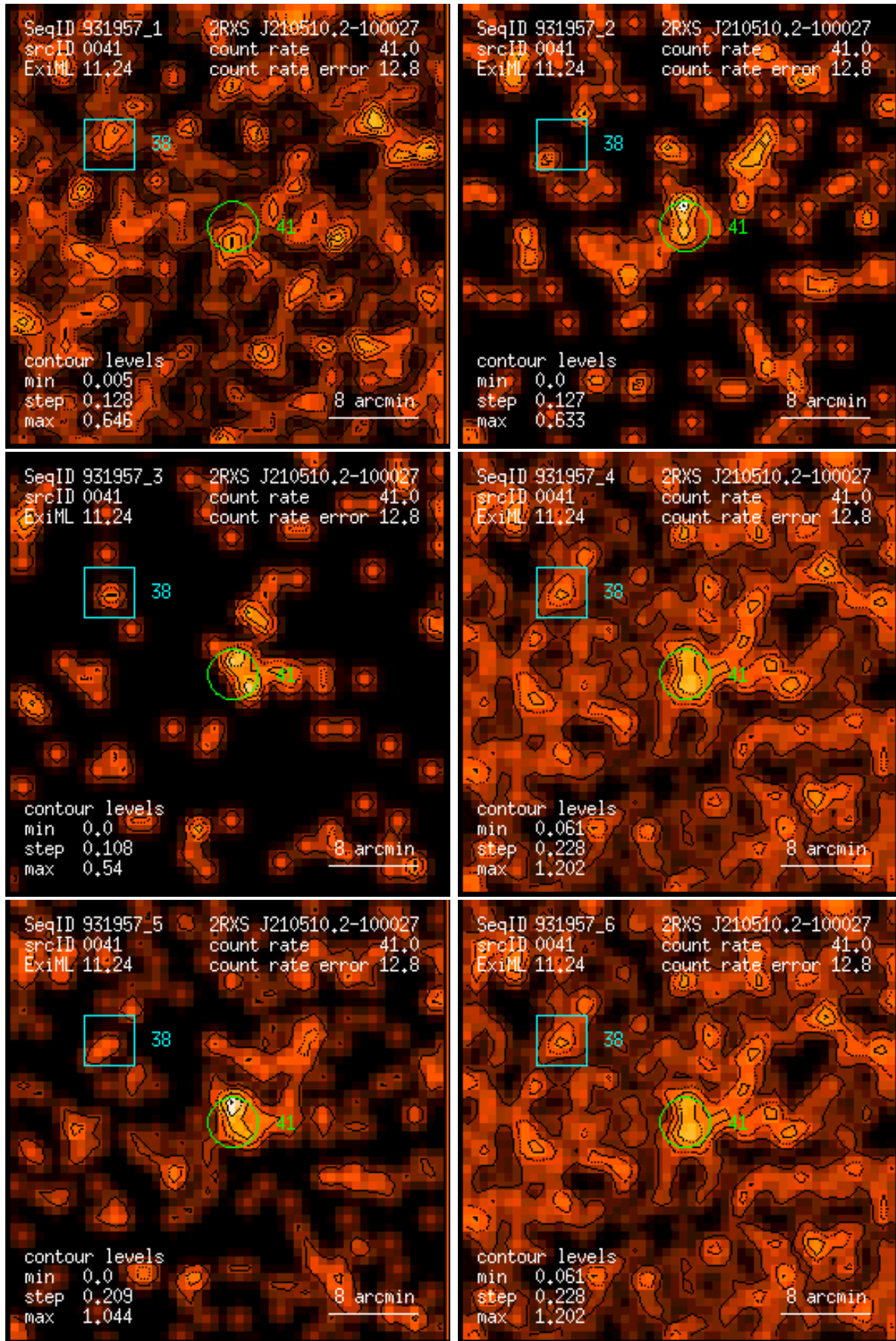
Figure 41: RASS 931957: detection 0041: band rate images, Gaussian filter: (1) PSPP channels 11 – 41, (2) 52 – 90, (3) 91 – 201, (4) 11 – 235, (5) 52 – 201, (6) 11 – 201. Broad band rates in counts/ks. Band rate contour levels in counts/ks/arcmin 2 .
