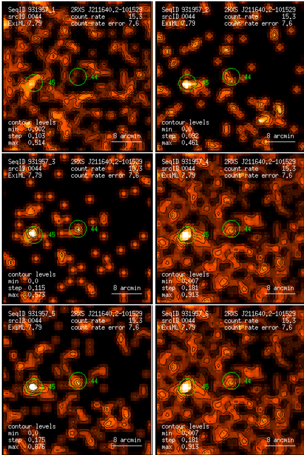
Figure 44: RASS 931957: detection 0044: band rate images, Gaussian filter: (1) PSPC channels 11 – 41, (2) 52 – 90, (3) 91 – 201, (4) 11 – 235, (5) 52 – 201, (6) 11 – 201. Broad band rates in counts/ks. Band rate contour levels in counts/ks/arcmin 2 .
