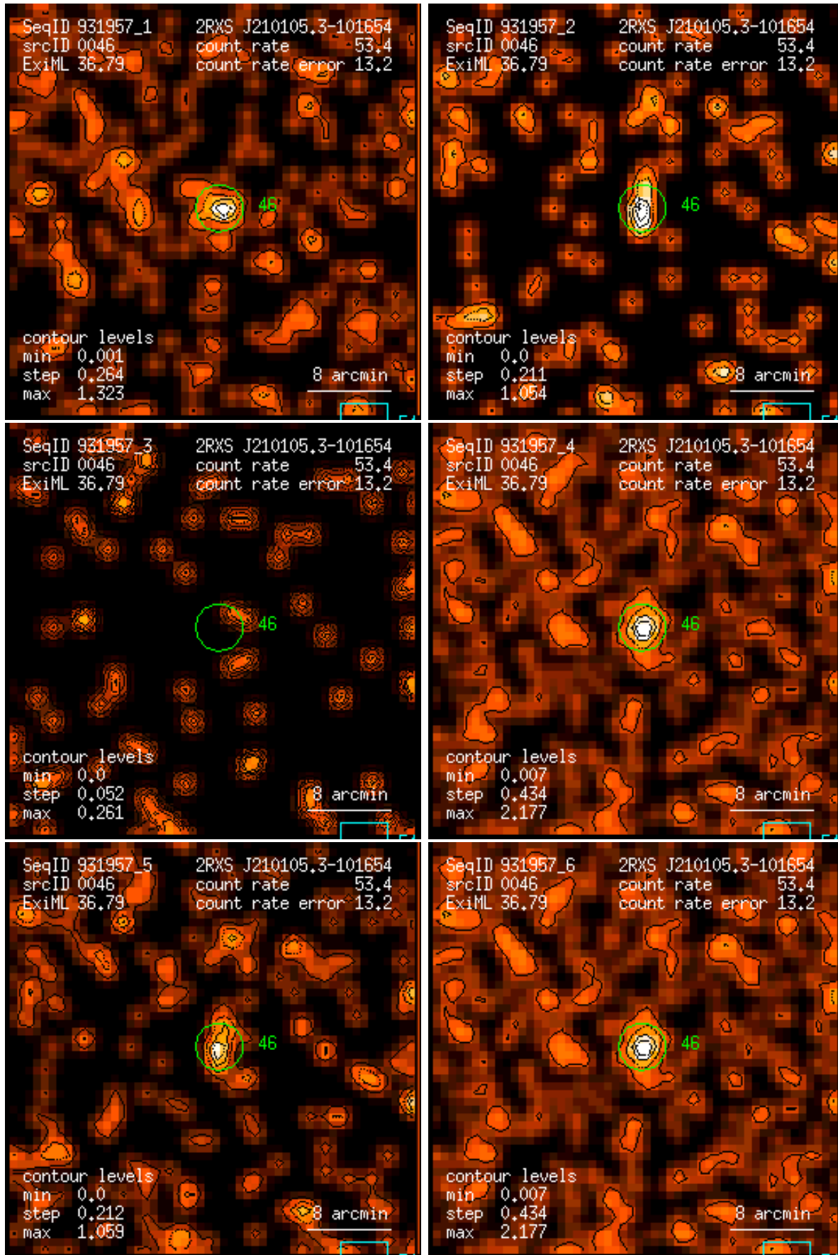
Figure 46: RASS 931957: detection 0046: band rate images, Gaussian filter: (1) PSPC channels 11 – 41, (2) 52 – 90, (3) 91 – 201, (4) 11 – 235, (5) 52 – 201, (6) 11 – 201. Broad band rates in counts/ks. Band rate contour levels in counts/ks/arcmin 2 .
